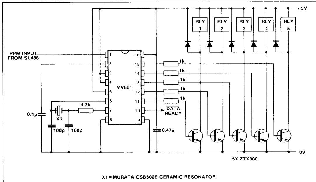
Fig.6 General purpose 5-function industrial remote control application (momentary mode)
