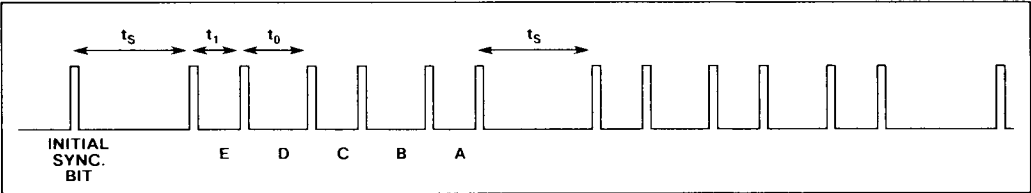
Fig.3 Typical Received PPM Data
