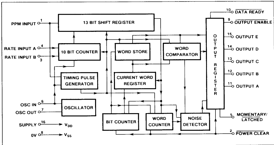
Fig.2 MV601 block diagram
