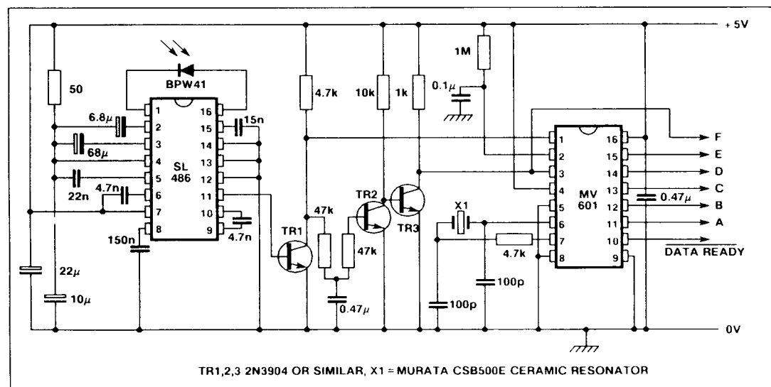
Fig.7 64-code application using a single MV601
