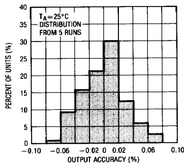
Distribution of Output Accuracy
