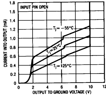
Shunt Characteristics
