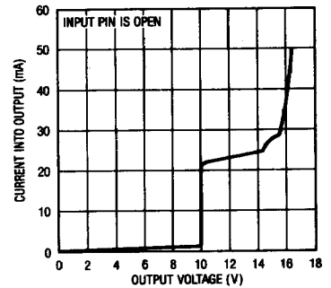
Shunt Mode Current Limit
