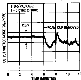
Noise Induced by Air Turbulence (TO-5 Package)
