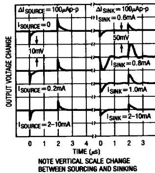
Load Transient Response C_{LOAD} = 0
