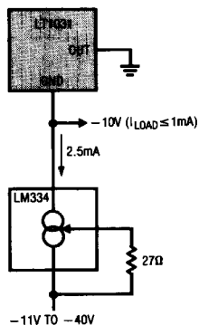
Negative Shunt Reference Driven by Current Source
