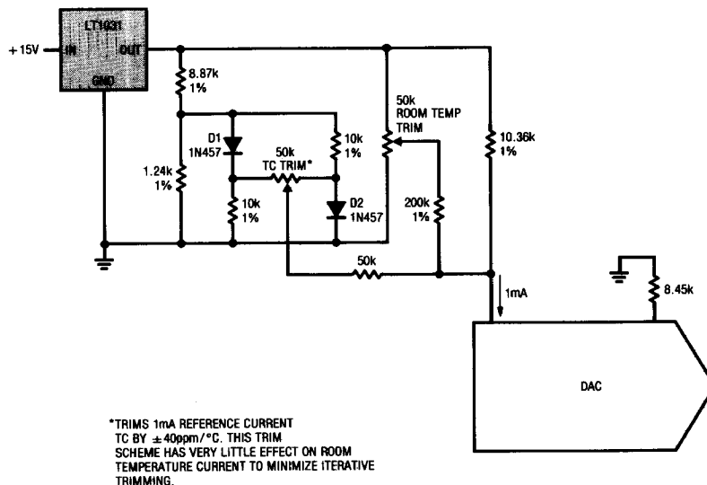
Precision DAC Reference with System TC Trim
