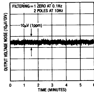
Output Noise 0.1Hz to 10Hz
