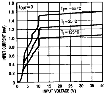
Input Supply Current
