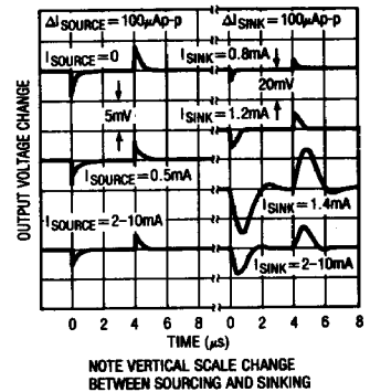
Load Transient Response C_{LOAD} = 1000\text{pF}
