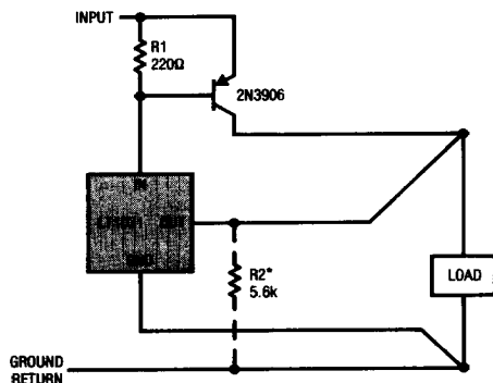
Series Mode with Boost Transistor
