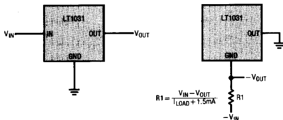
Basic Positive and Negative Connections
