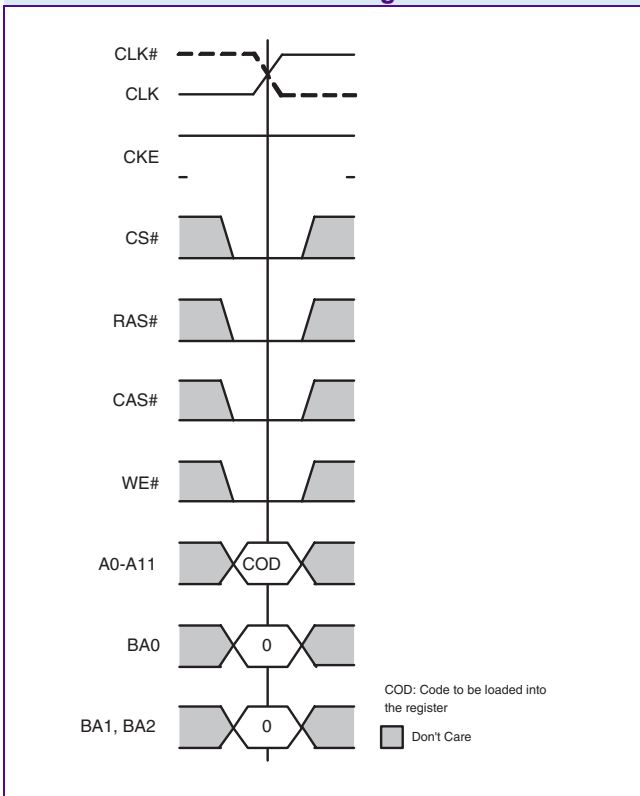
Mode Register Set Command
