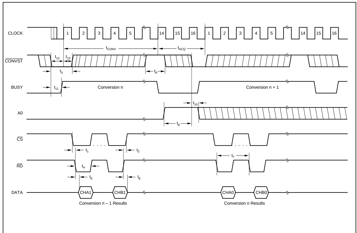
FIGURE 9. Reading and Writing to the ADS7862 During the Same Cycle.
