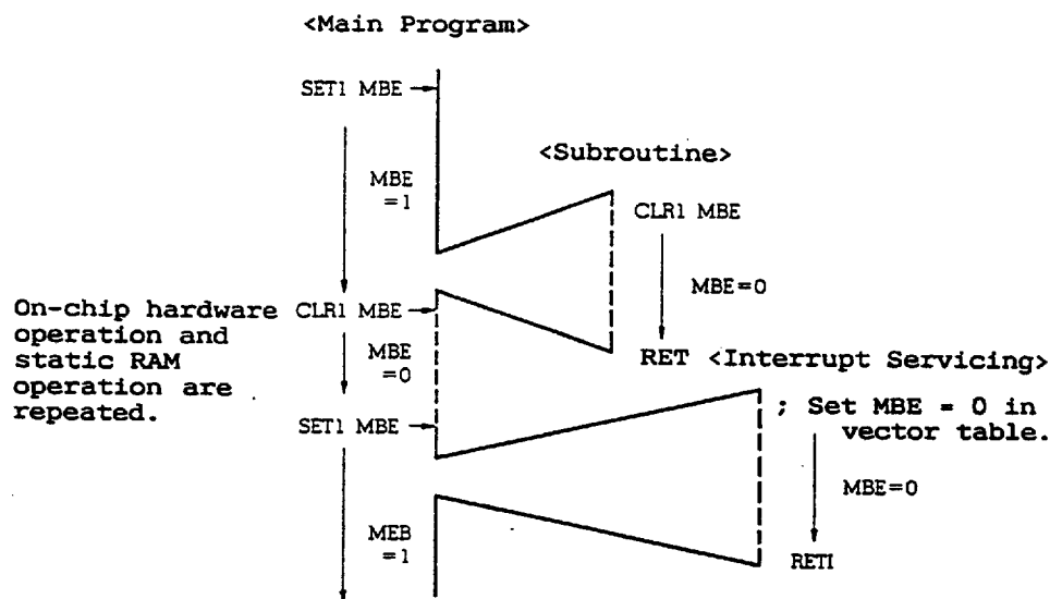
Figure 3-1 MBE = 0 Mode and MBE = 1 Mode Distinction
