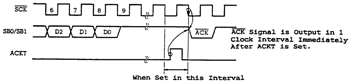
Figure 5-55 ACKT Operation
