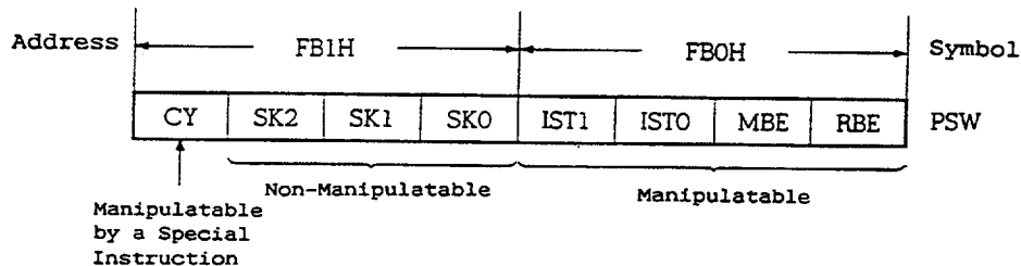
Figure 4-11 Program Status Word Configuration
