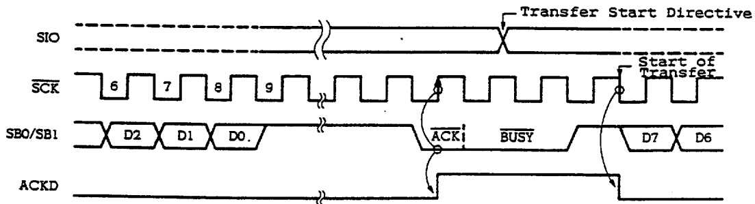
Figure 5-58 BSYE Operation
