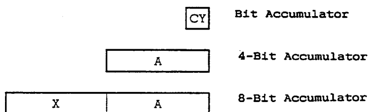
Figure 4-7 Accumulator
