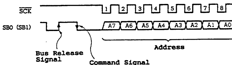
Figure 5-47 Address
