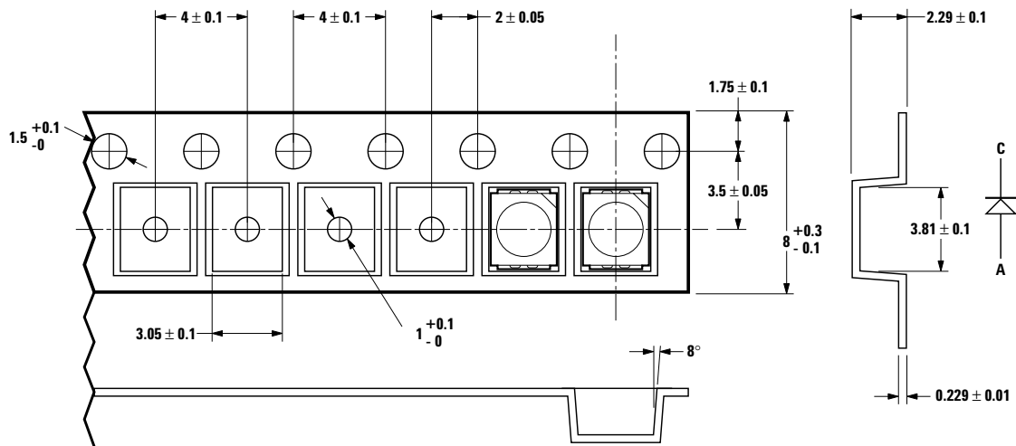
Figure 10. Tape dimension.
