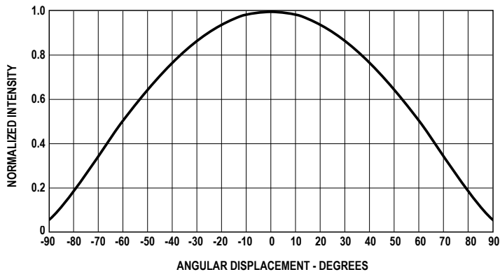
Figure 5. Radiation pattern.
