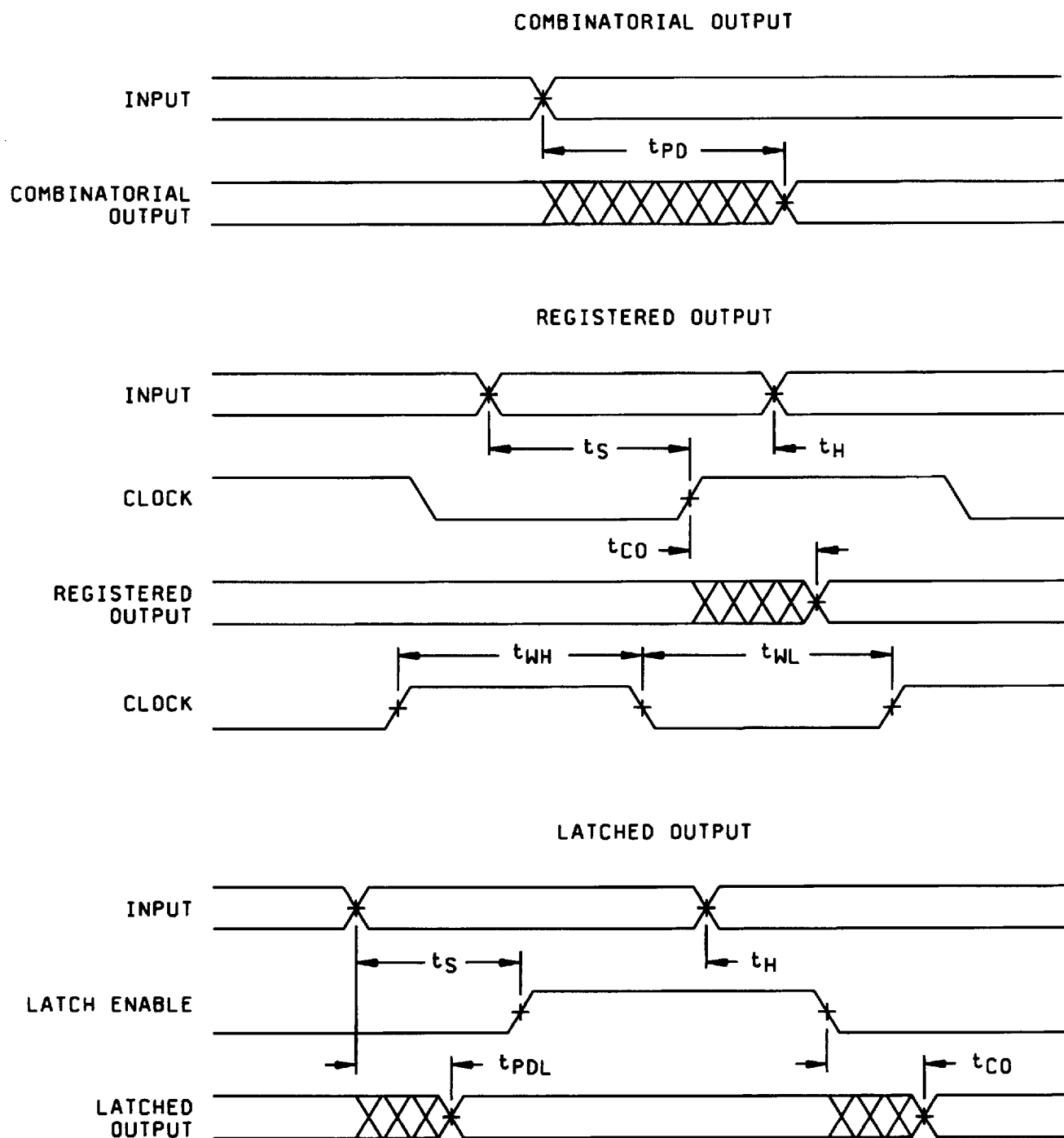
FIGURE 4. Switching waveforms.
