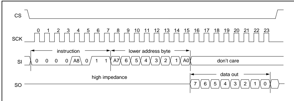
FIGURE 3-2: READ SEQUENCE
