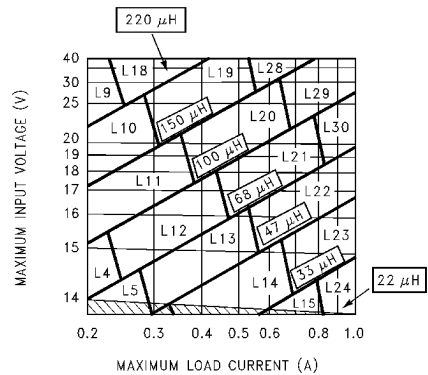
FIGURE 6. LM2675-12
