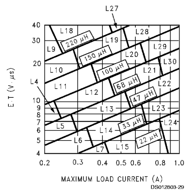
FIGURE 7. LM2675-ADJ
