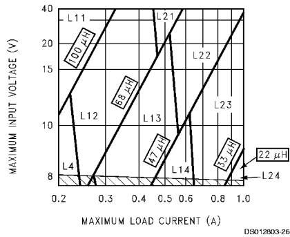
FIGURE 4. LM2675-3.3
