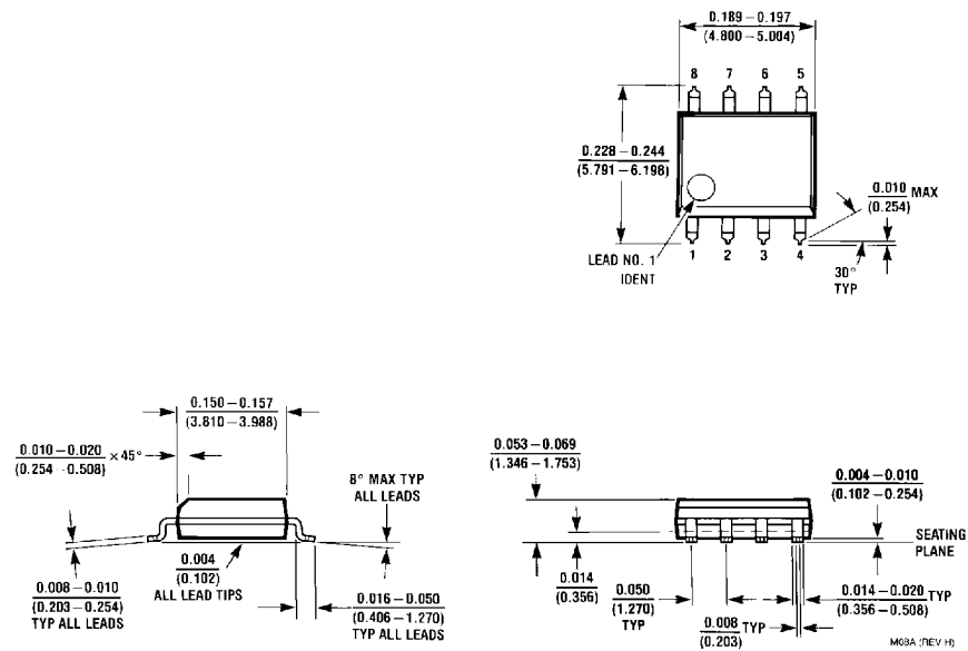
8-Lead (0.150" Wide) Molded Small Outline Package, JEDEC Order Number LM2675M-3.3, LM2675M-5.0, LM2675M-12 or LM2675M-ADJ NS Package Number M08A
