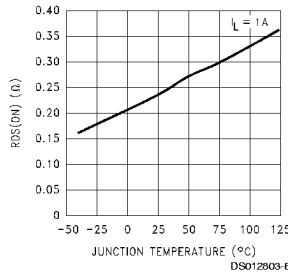
Drain-to-Source Resistance
