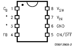
8-Lead Package Top View
