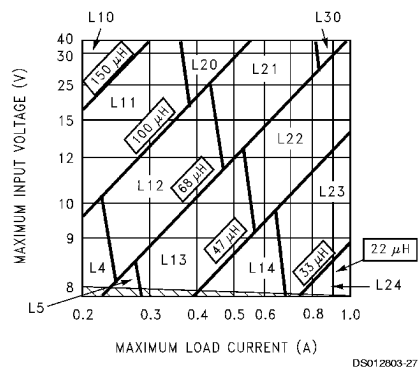
FIGURE 5. LM2675-5.0
