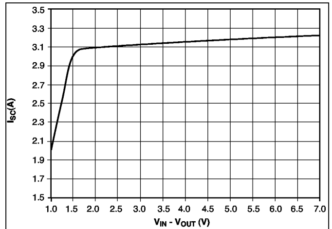
Short Circuit Current vs V_{IN} - V_{OUT}
