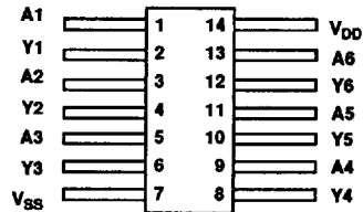
14-Lead Flatpack Top View
