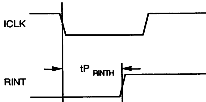
Fig. 16 RBOC Output Timing
