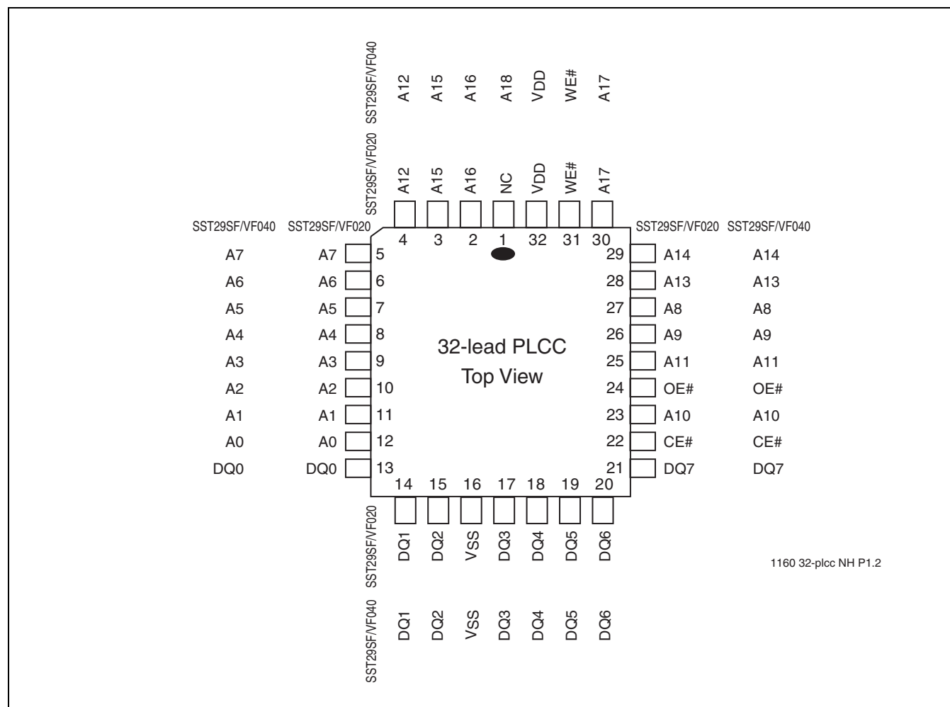
FIGURE 2: Pin Assignments for 32-lead PLCC
