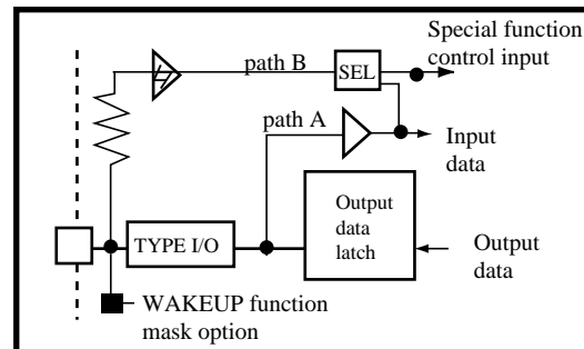
TYPE I/O-L
