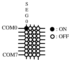
(3) LCD waveform :
