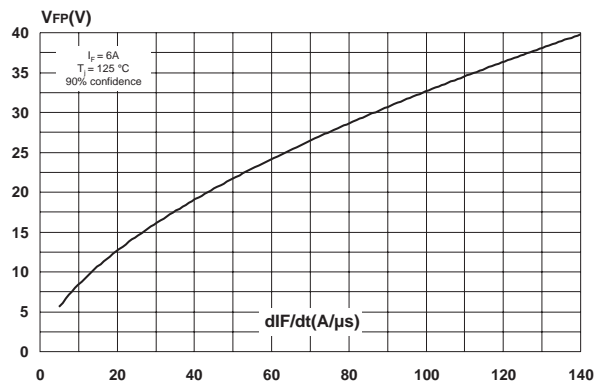
Fig. 9-1: Forward recovery time versus dI/dt (damper diode).
