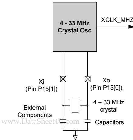
Figure 6-2. MHzECO Block Diagram
