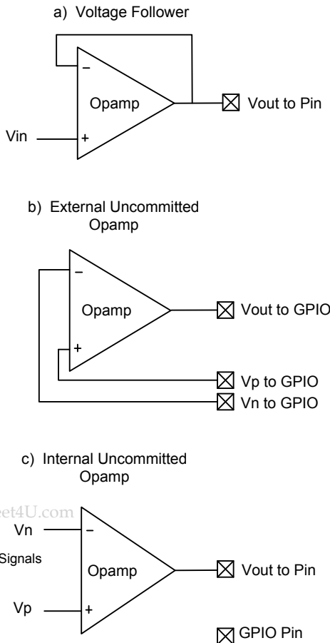
Figure 8-6. Opamp Configurations
