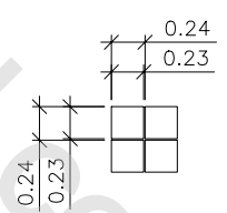
Detail of dots Scale: 20/1
