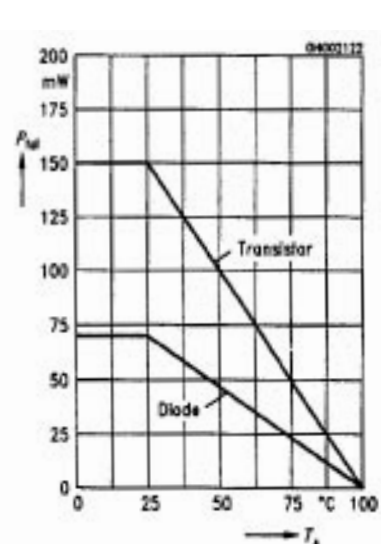
Figure 8. Permissible power dissipation P_{TOT}=f(T_A)
