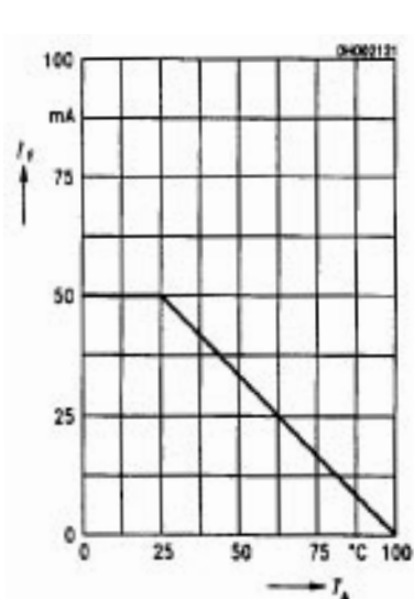
Figure 7. Permissible forward current diode I_F=f(T_A)
