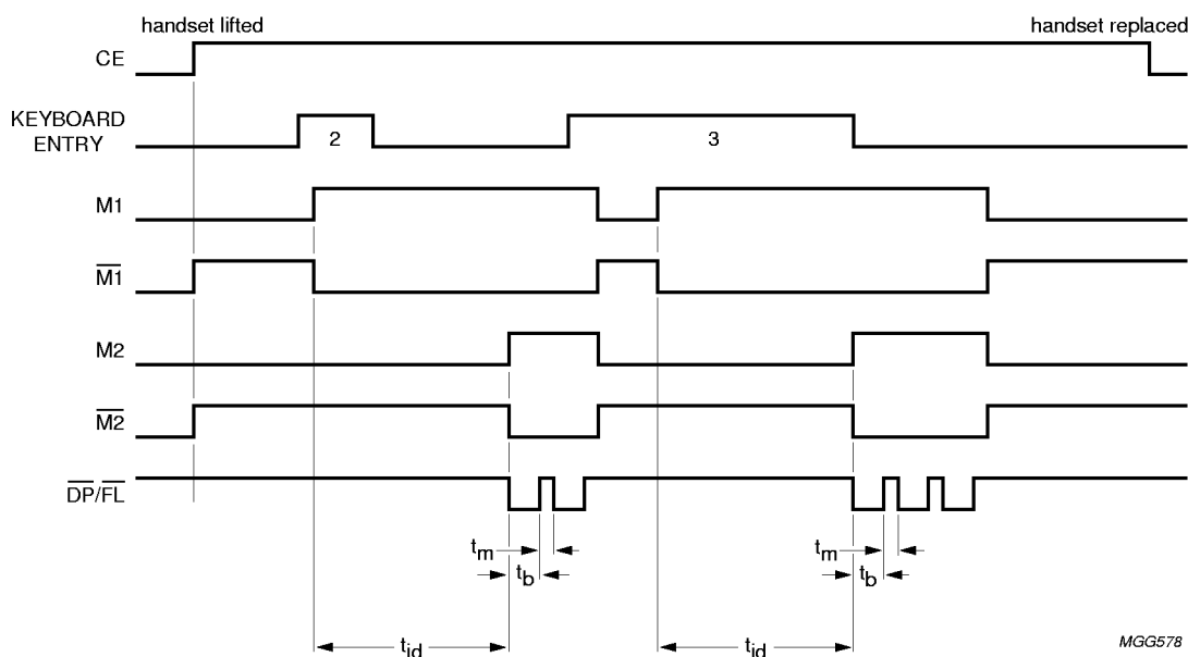
Fig.8 Timing diagram in pulse mode, showing \overline{\text{DP/FL}} and MUTE outputs.
