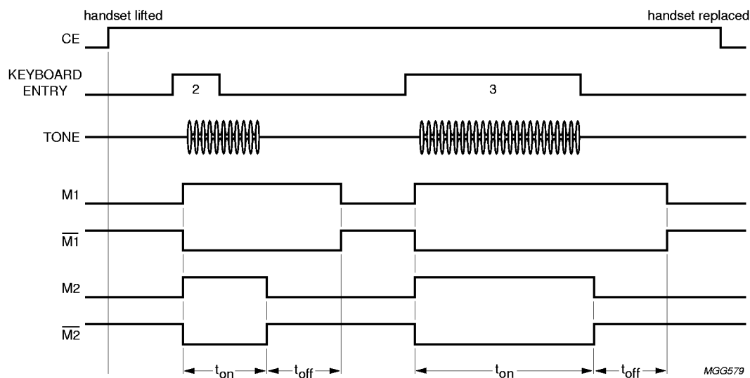
Fig.9 Timing diagram in DTMF mode, showing MUTE outputs.
