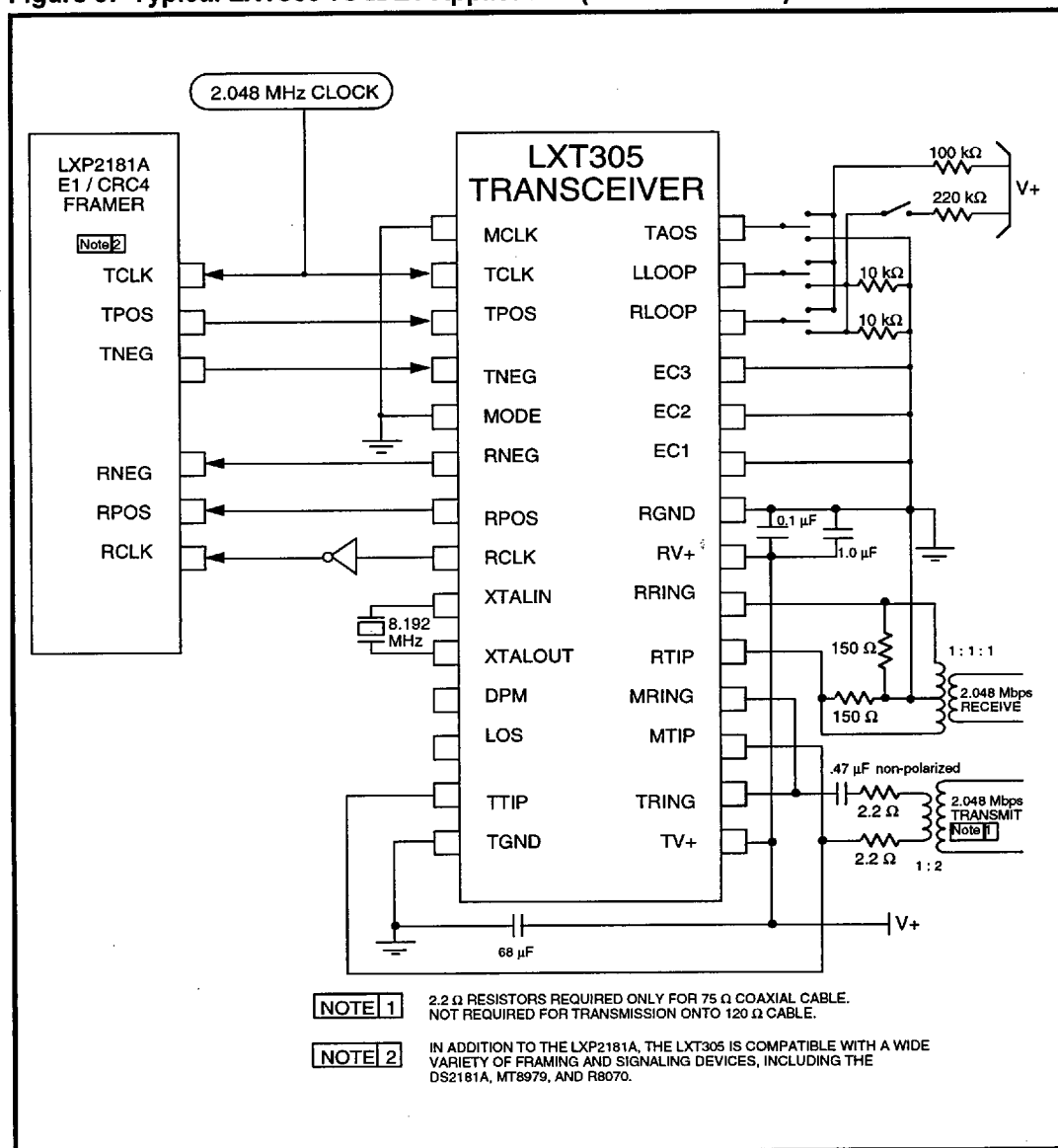
Figure 5: Typical LXT305 75 \Omega E1 Application (Hardware Mode)
