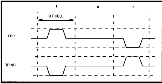
Figure 2: 50% AMI Coding Diagram
