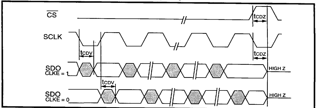
Figure 9: LXT305 Serial Data Output Timing Diagram
