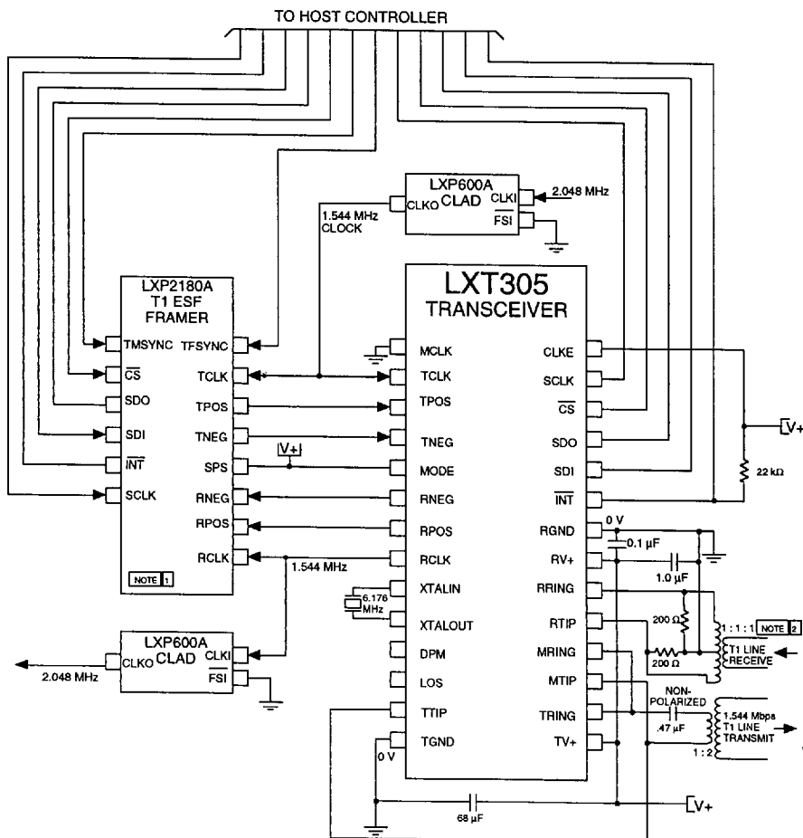
Figure 4: Typical LXT305 1.544 Mbps T1 Application (Host Mode)
