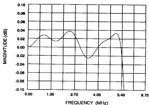
Fig. 4 Frequency Response of Luminance Interpolation Filter (Sampling at f_s = 27 MHz)
