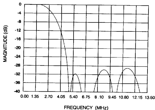
Fig. 5 Frequency Response of Chrominance Interpolation Filter (Sampling at f_s = 27 MHz)
