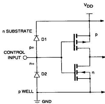
Fig. 2a Equivalent Input Circuit
