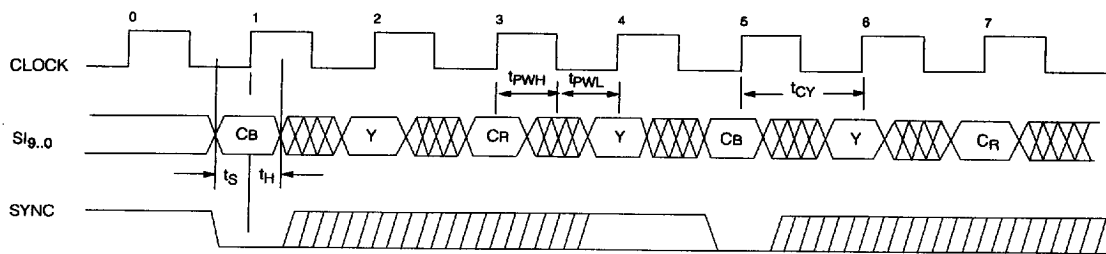
Fig. 9 Operation of SYNC Control Signal
