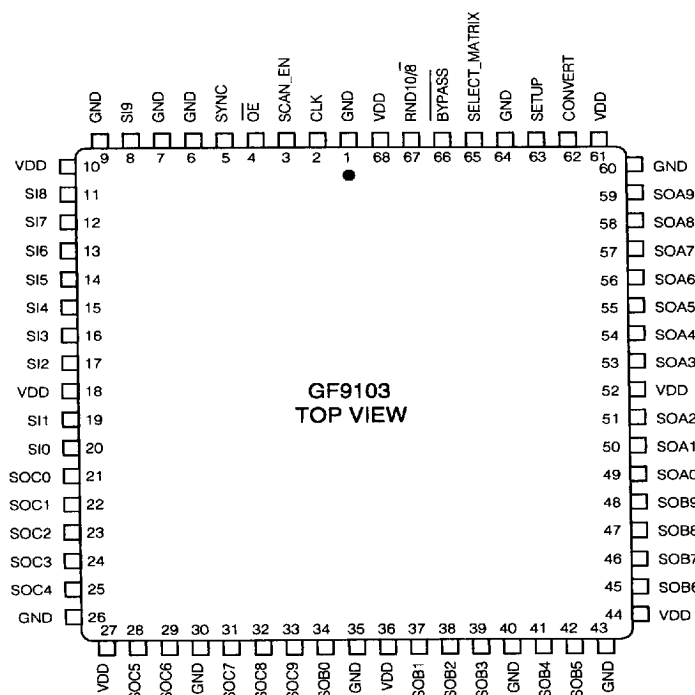
Fig. 1 GF9103 Pin Connections
