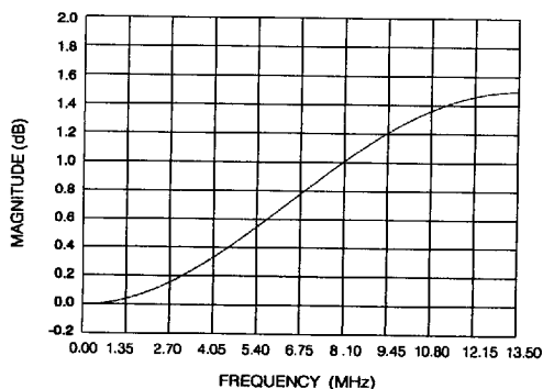
Fig. 7 SIN X/X Compensation Filter Frequency Response (Sampling at f_s = 27 MHz)
