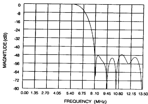
Fig. 3 Frequency Response of Luminance Interpolation Filter (Sampling at f_s = 27 MHz)
