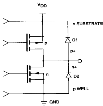
Fig. 2b Equivalent Output Circuit
