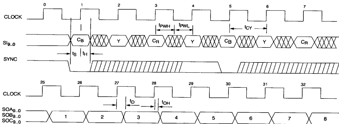
Fig. 11 Input/Output Timing. \overline{\text{BYPASS}} = 1 .
