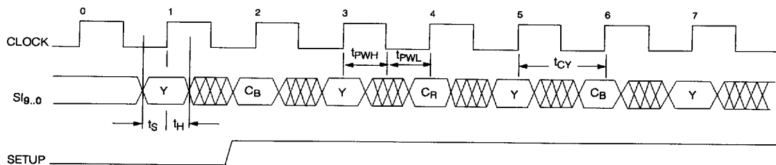
Fig. 10 Operation of SETUP Control Signal
