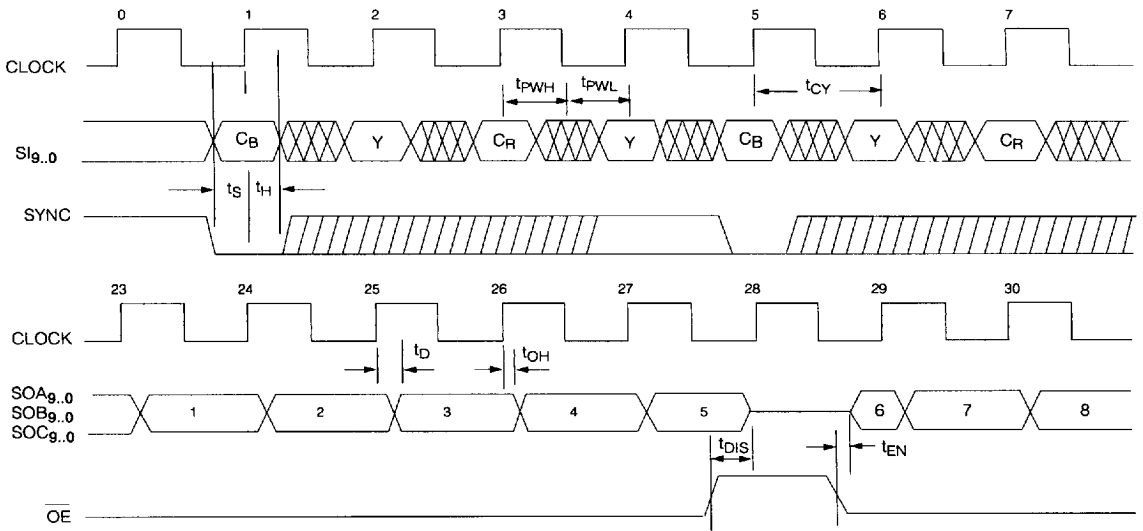
Fig. 12 Input/Output Timing. BYPASS = 0.
