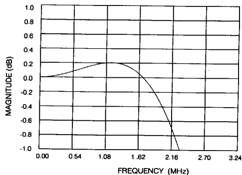
Fig. 6 Frequency Response of Chrominance Interpolation Filter (Sampling at f_s = 27 MHz)
