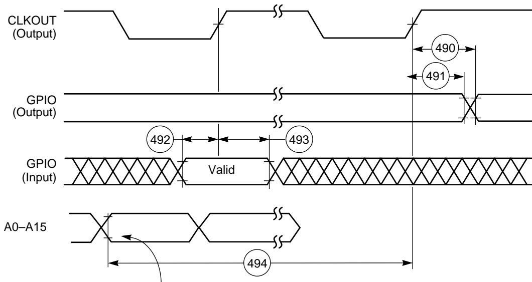
Figure 2-24 GPIO Timing
