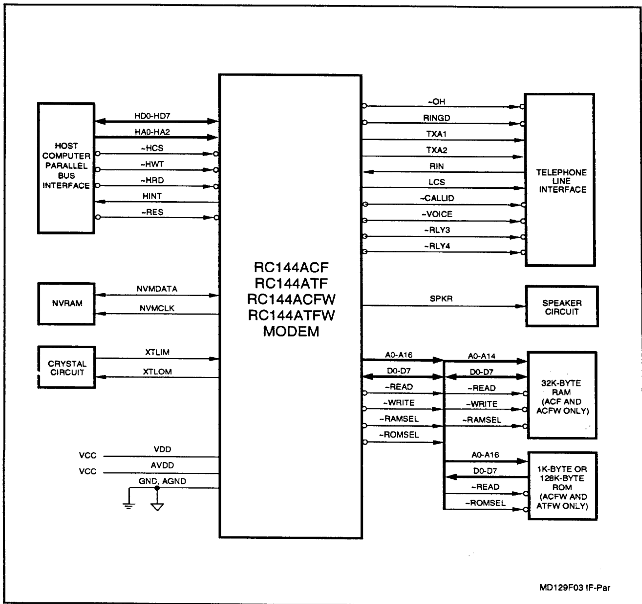
Figure 3. Hardware Interface Signals - Parallel Interface
