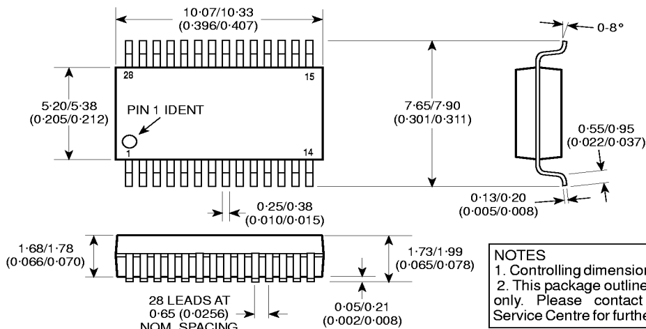
28-LEAD SHRUNK MINIATURE PLASTIC DIL (SSOP) - NP28
