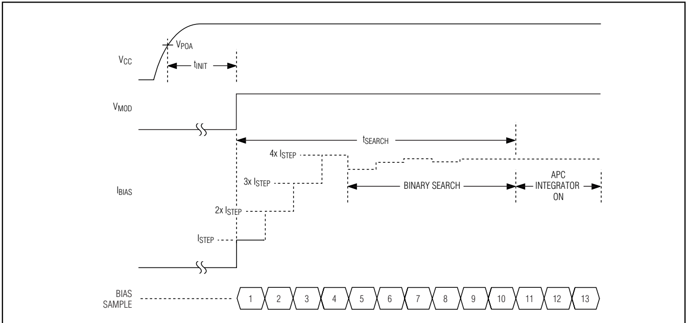
Figure 1. Power-Up Timing
