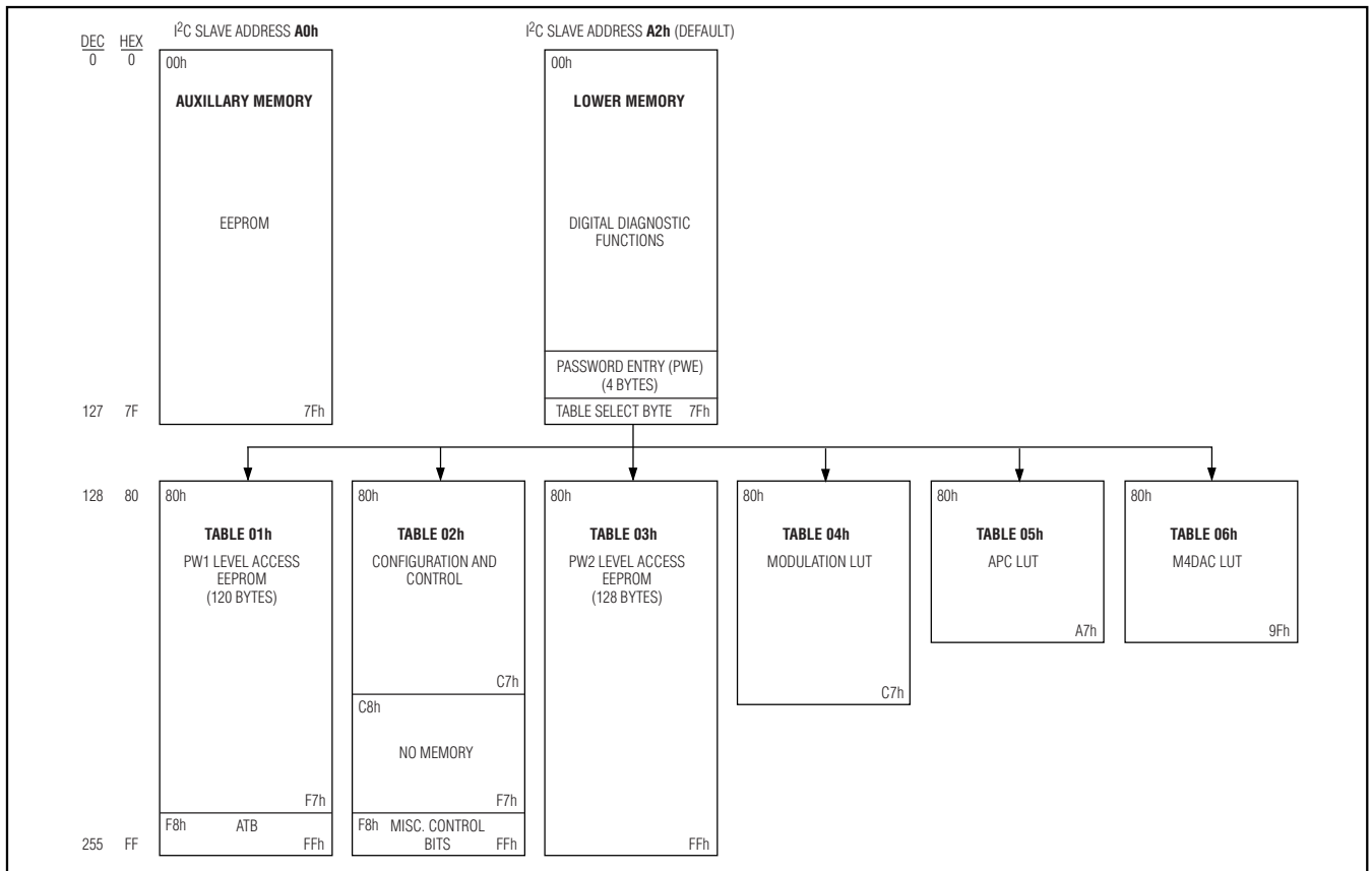
Figure 8. Memory Map
