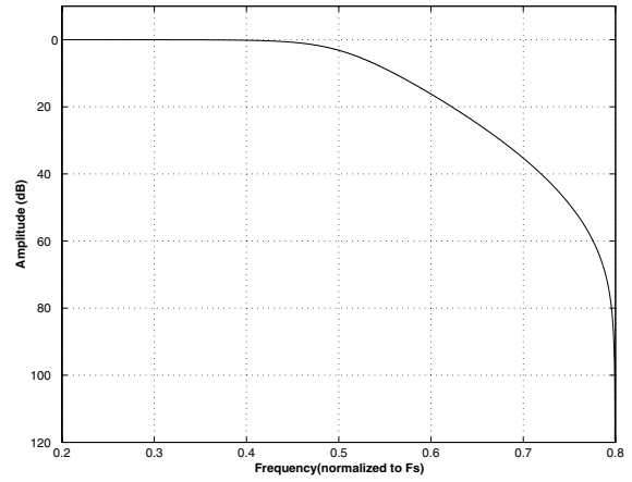
Figure 25. Double Speed (slow) Transition Band
