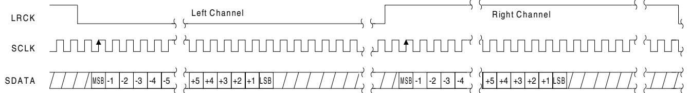
Figure 5. Format 1, I 2 S up to 24-Bit Data
