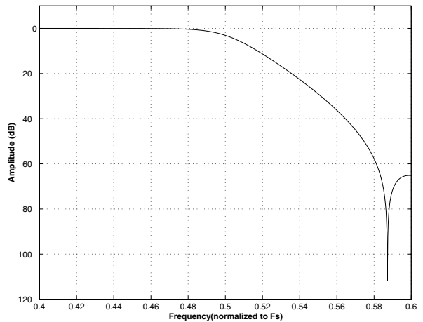
Figure 17. Single Speed (slow) Transition Band
