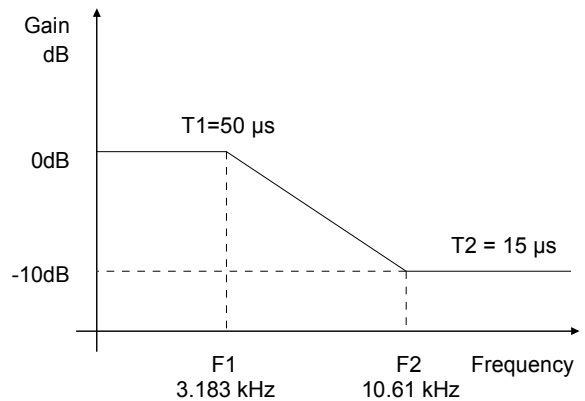
Figure 10. De-Emphasis Curve
