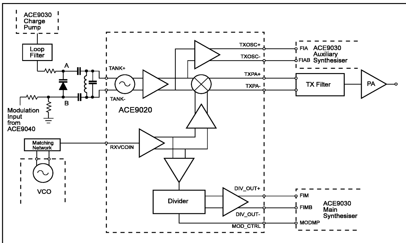
Fig. 4 Application Diagram
