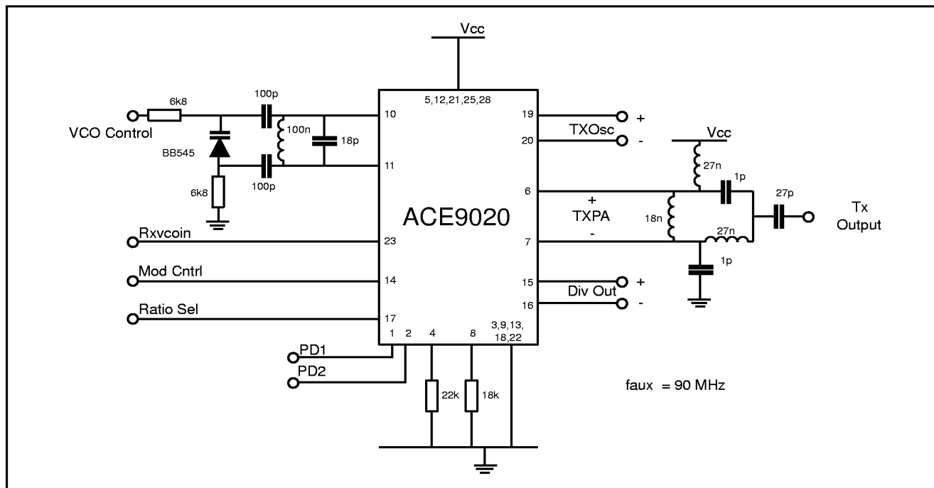
Fig. 3 ACE9020 Test circuit
