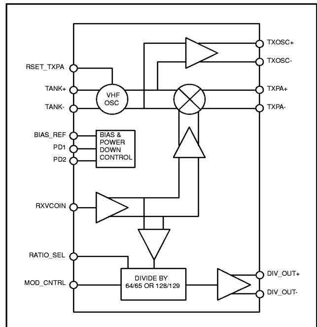
Fig. 2 ACE9020 simplified block diagram
