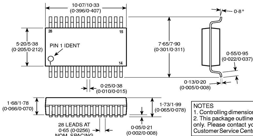
28-LEAD SHRUNK MINIATURE PLASTIC DIL (SSOP) - NP28
