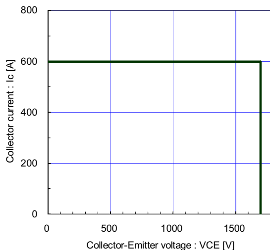
Reverse bias safe operating area (max.) +V_{GE}=15V, -V_{GE} \le 15V, R_g \ge 1.5\Omega, T_j \le 125^\circ C
