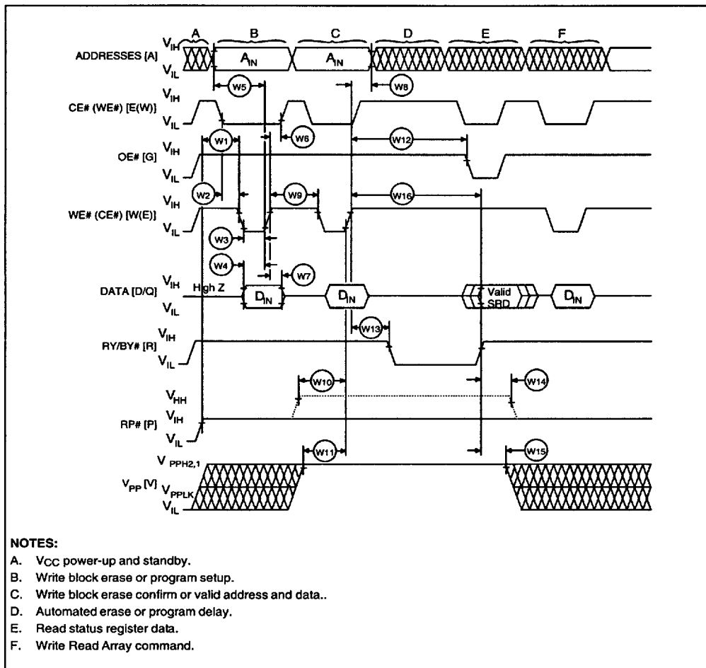
Figure 17. AC Waveform for Write Operations
