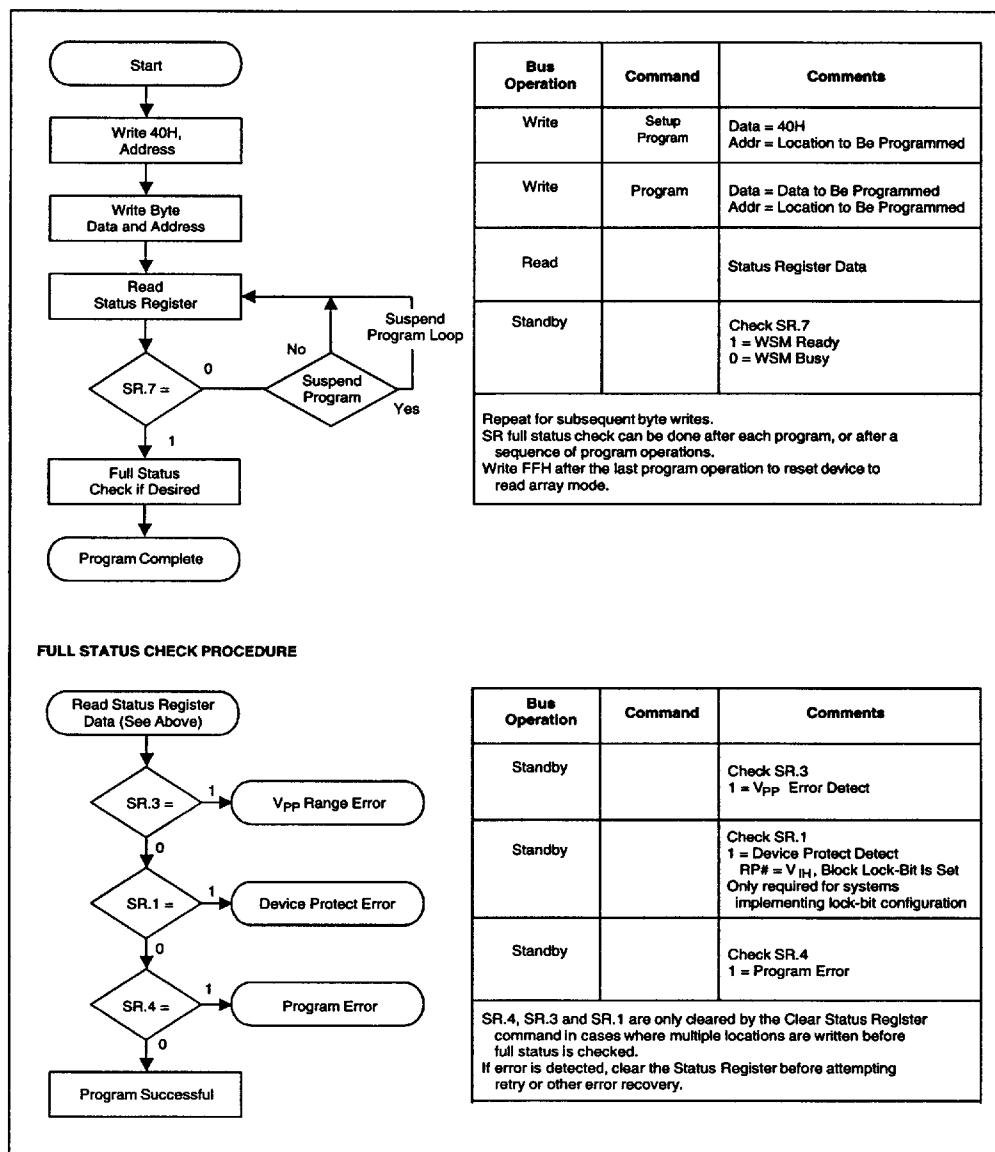
Figure 7. Automated Program Flowchart
