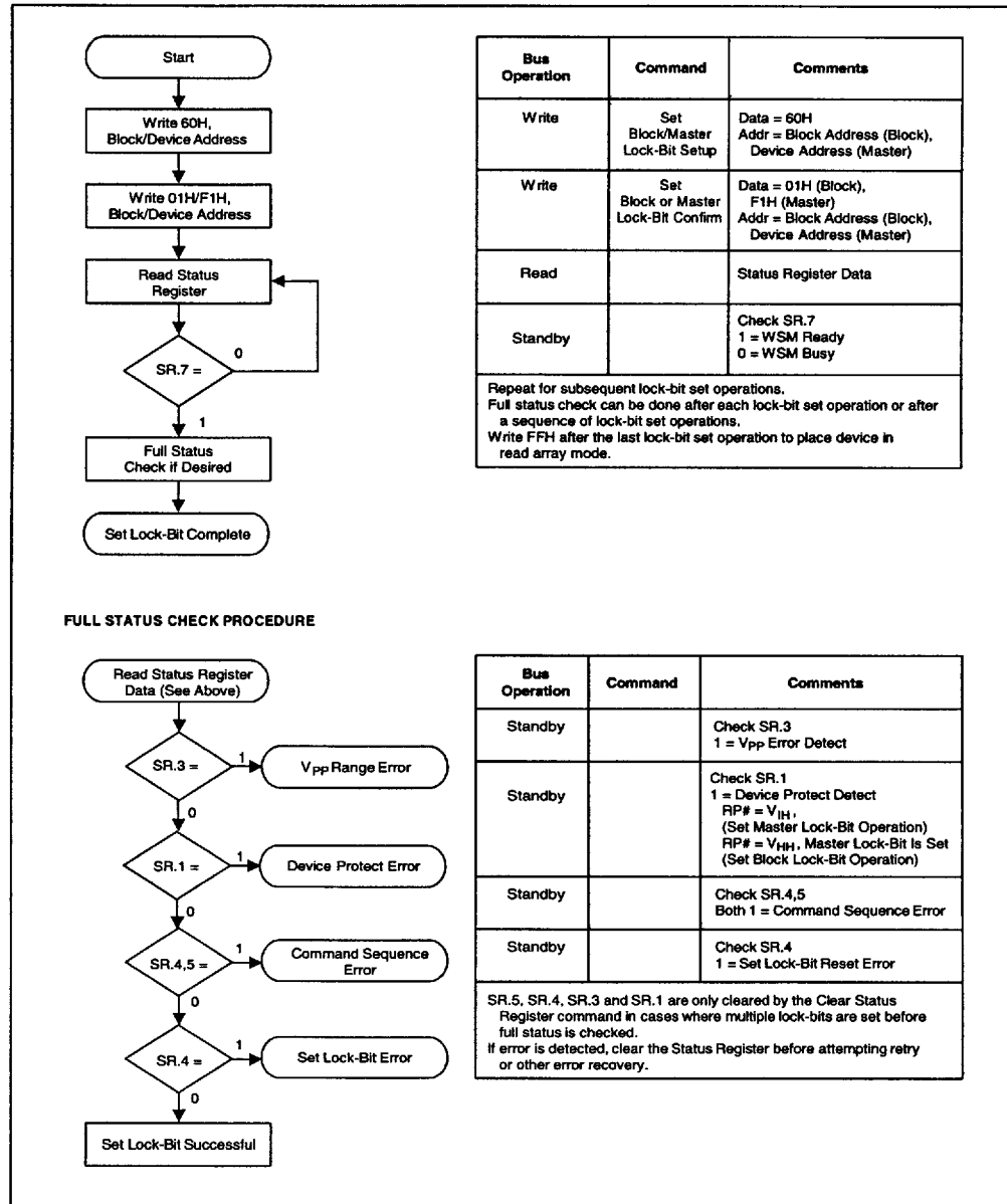
Figure 10. Set Block and Master Lock-Bit Flowchart
