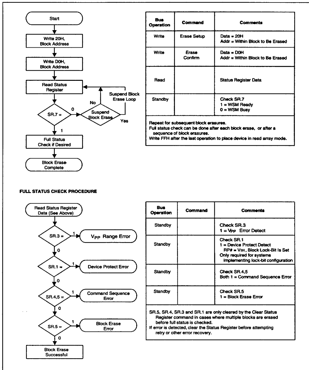
Figure 6. Automated Block Erase Flowchart
