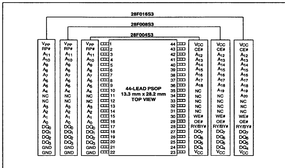
Figure 3. PSOP 44-Lead Pinout
