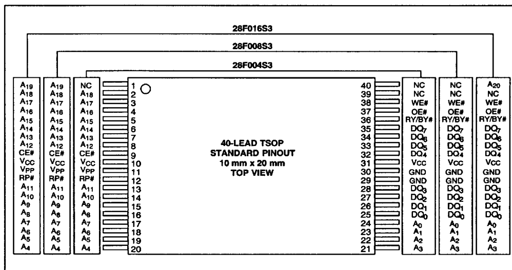
Figure 2. TSOP 40-Lead Pinout
