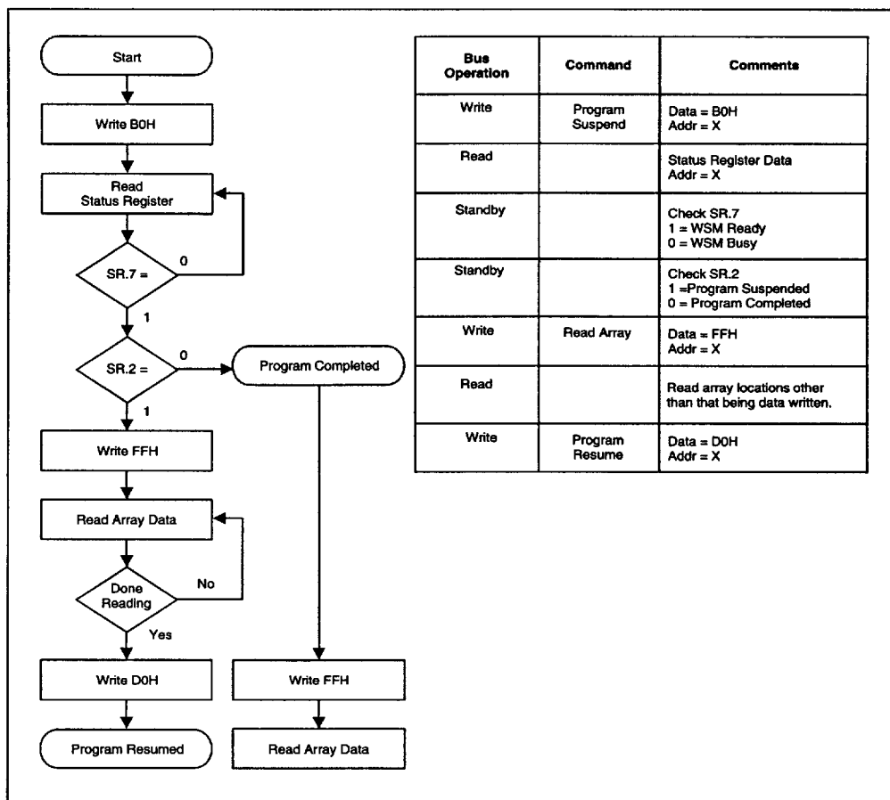
Figure 9. Program Suspend/Resume Flowchart
