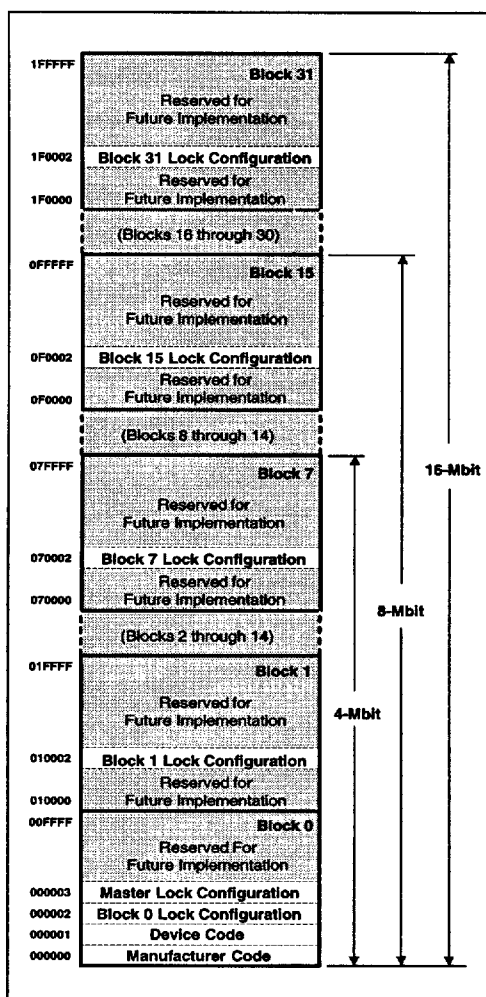
Figure 5. Device Identifier Code Memory Map
