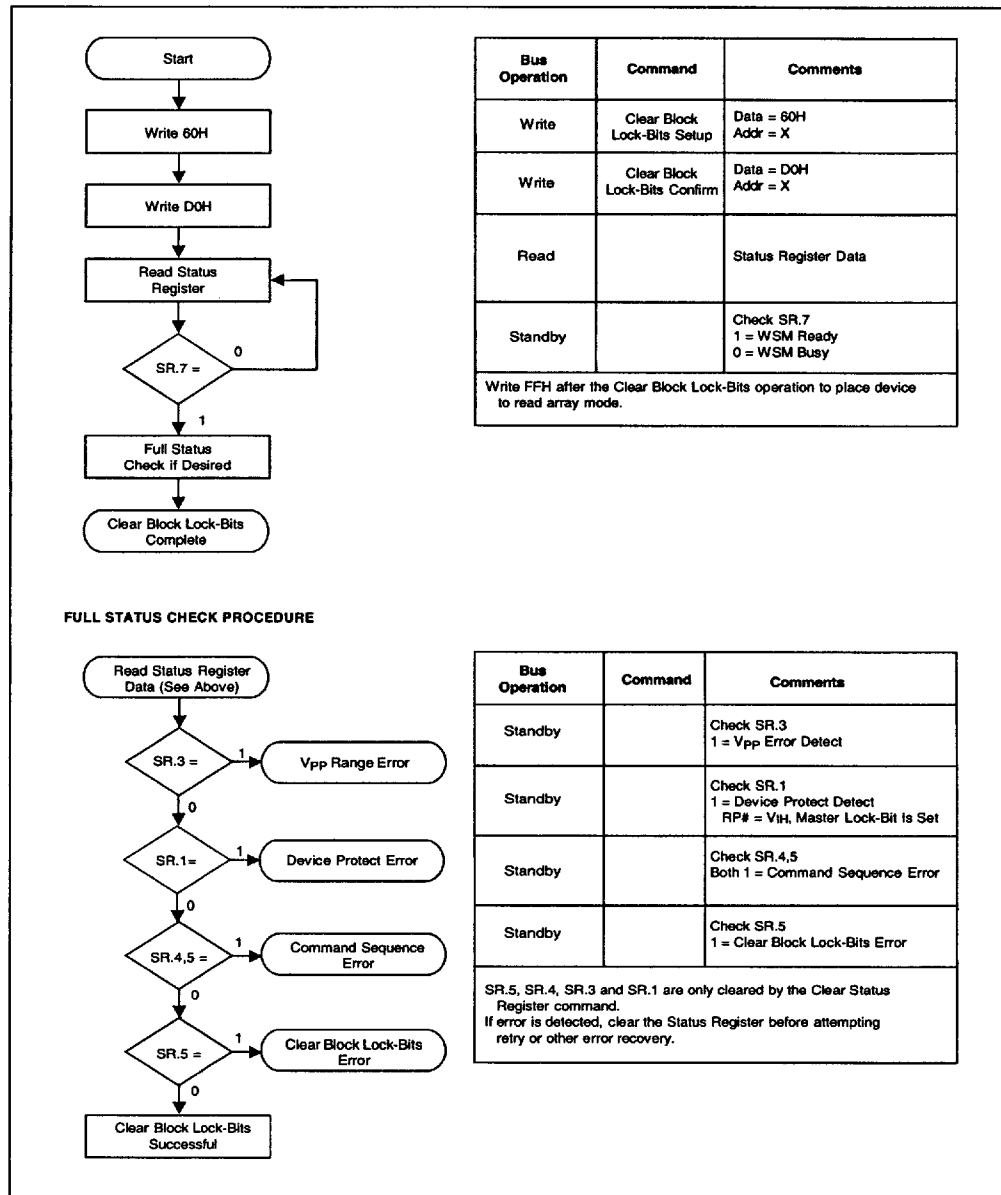
Figure 11. Clear Block Lock-Bits Flowchart
