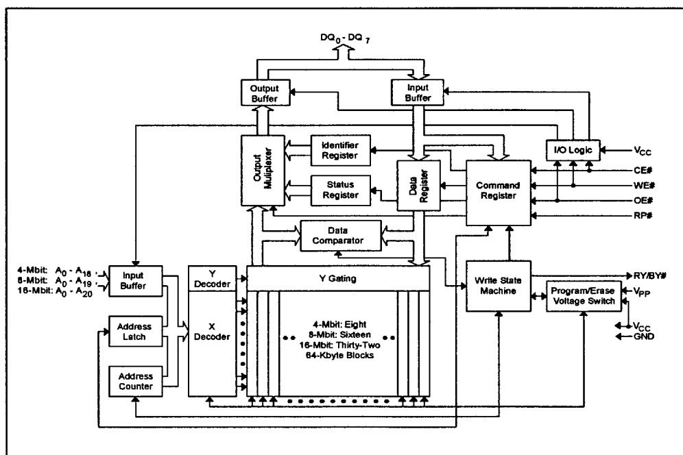
Figure 1. Block Diagram
