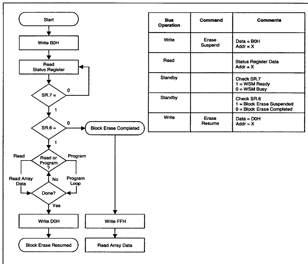
Figure 8. Block Erase Suspend/Resume Flowchart
