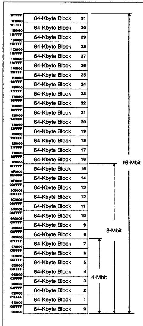
Figure 4. Memory Map
