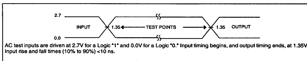
Figure 12. Transient Input/Output Reference Waveform for V_{CC} = 2.7V-3.6V
