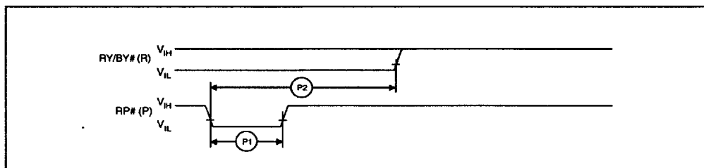
Figure 16. AC Waveform for Reset Operation
