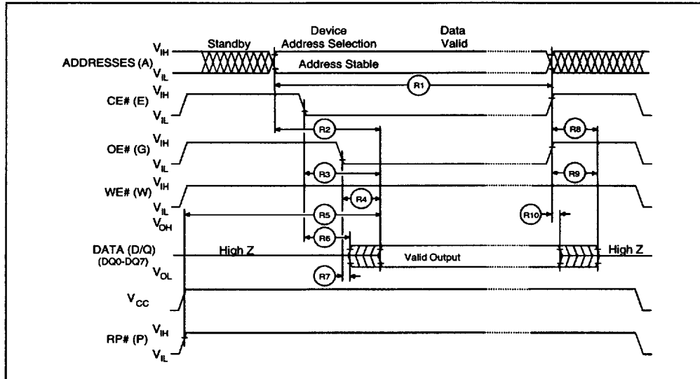
Figure 15. AC Waveform for Read Operations
