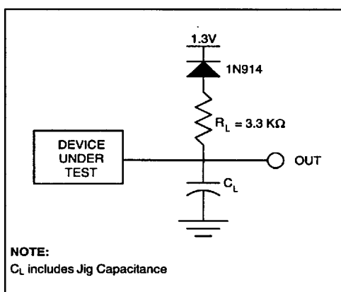
Figure 14. Transient Equivalent Testing Load Circuit
