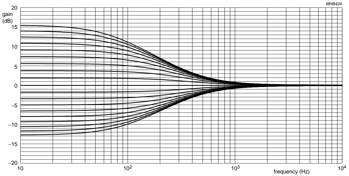
Fig.19 Bass curve with 1 \times 47 nF external, between pin 31 and pin 32, BSYB = 0 and BSYC = 0.
