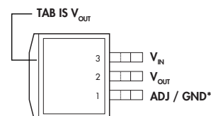
DD & DL PACKAGES (Top View)
