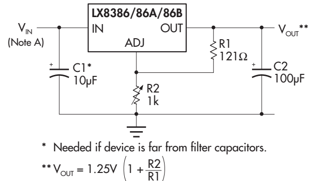
FIGURE 5 — 1.2V - 8V Adjustable Regulator
