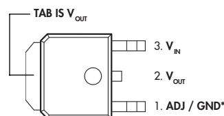
DT PACKAGE (D-Pak) (Top View)
