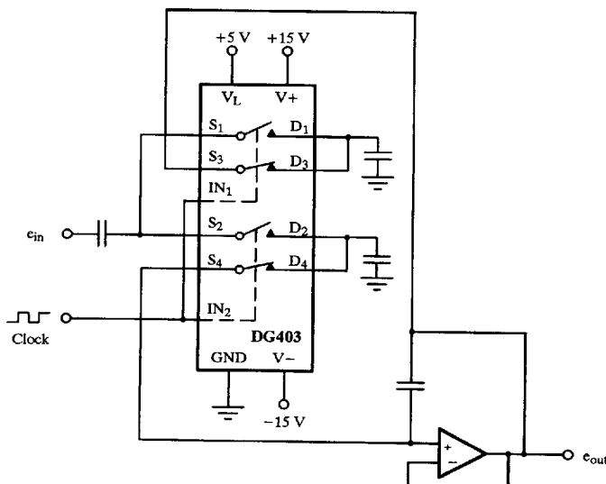
Figure 11. Band-Pass Switched Capacitor Filter
