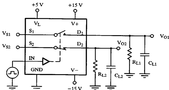
Figure 2. Switching Time
