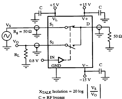
Figure 7. Crosstalk
