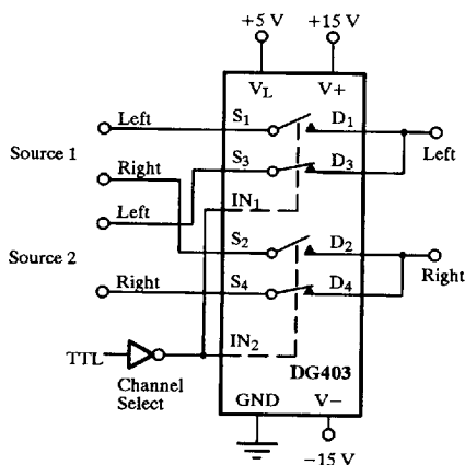
Figure 9. Stereo Source Selector
