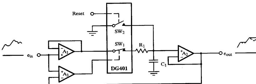
Figure 12. Positive Peak Detector
