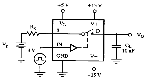
Figure 4. Charge Injection
