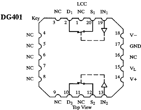
Two SPST Switches per Package
