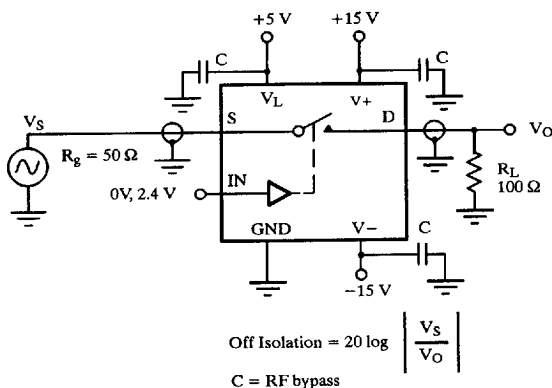
Figure 5. Off Isolation
