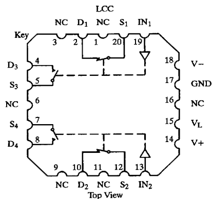
Two SPDT Switches per Package
