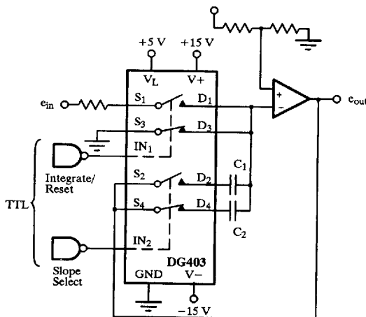
Figure 10. Dual Slope Integrator
