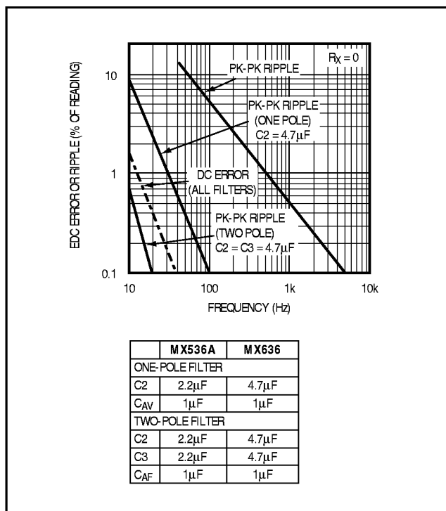
Figure 9. Performance Features of Various Filter Types for MX536A/MX636
