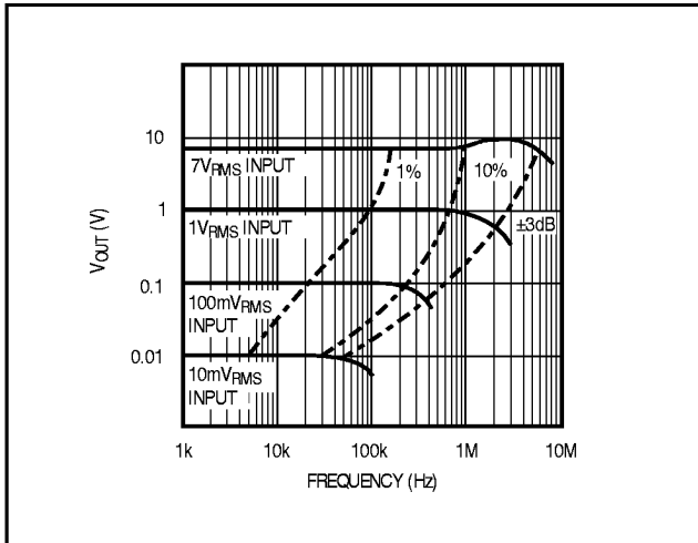
Figure 11. MX536A High-Frequency Response
