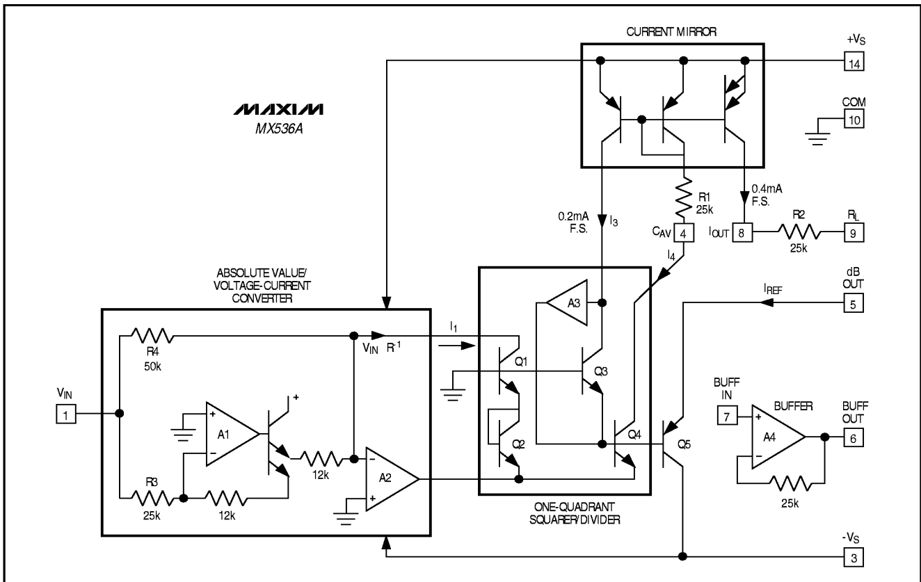
Figure 1. MX536A Simplified Schematic
