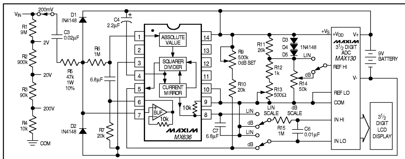
Figure 13. Portable High-Z Input RMS DPM and dB Meter
