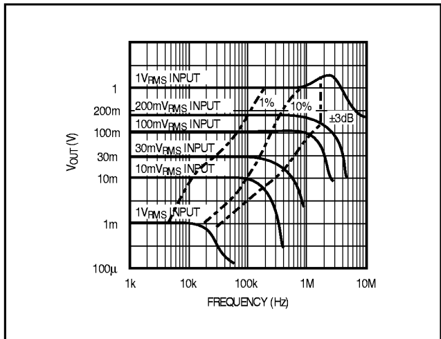
Figure 12. MX636 High-Frequency Response
