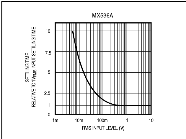
Figure 6a. MX536A Settling Time vs. Input Level
