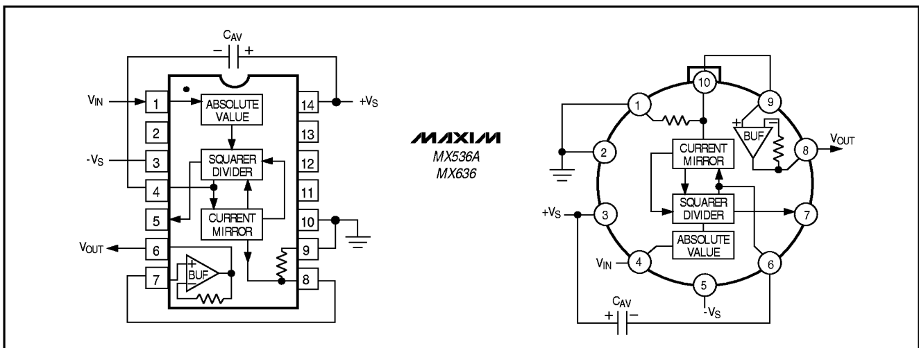
Figure 2. MX536A/MX636 Standard RMS Connection
