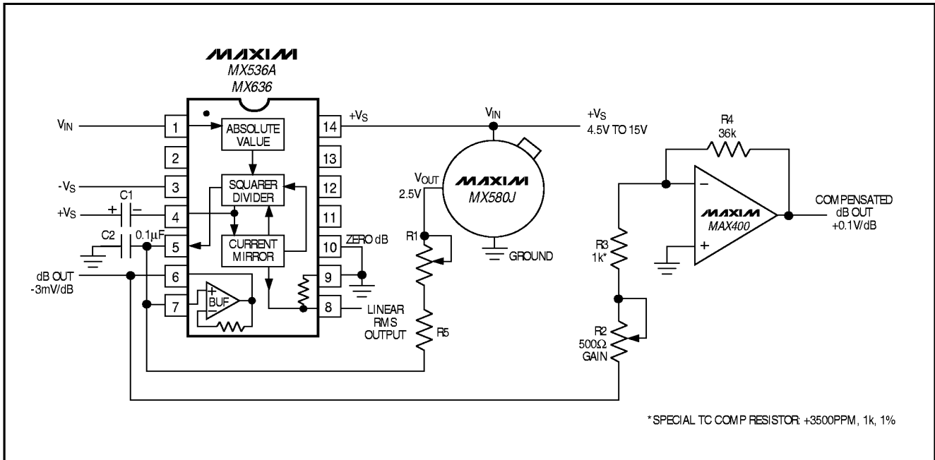
Figure 10. dB Connection
