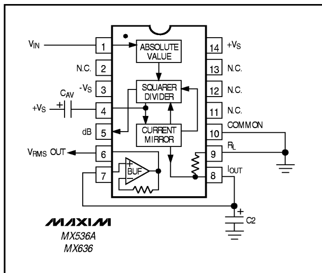
Figure 7. MX536A/MX636 with a One-Pole Output Filter
