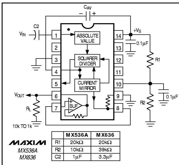
Figure 5. Single-Supply Operation
