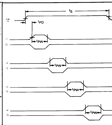
Figure 7. WD2143-03 TIMING DIAGRAM
