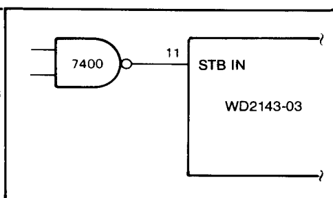
Figure 3. TTL SQUARE WAVE OPERATION
