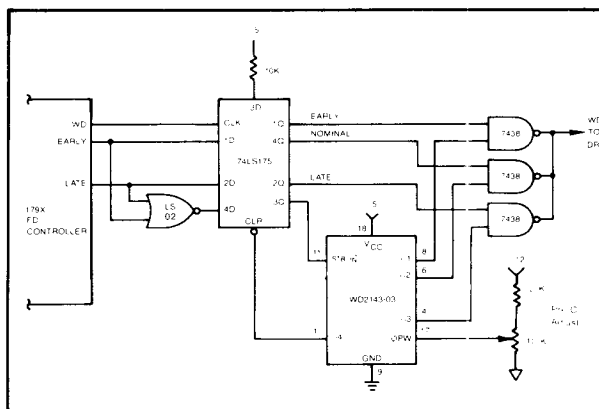
Figure 6. WRITE PRECOMP FOR FLOPPY DISK
