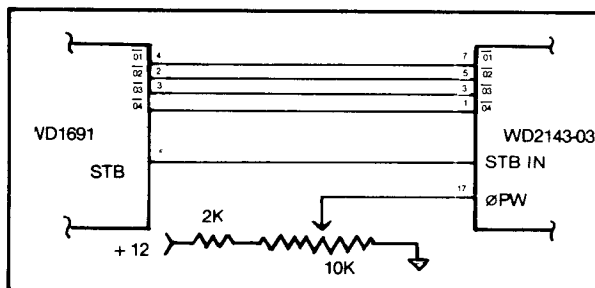
Figure 2. WRITE PRECOMP OPERATION WITH F.S.L. WD1691
