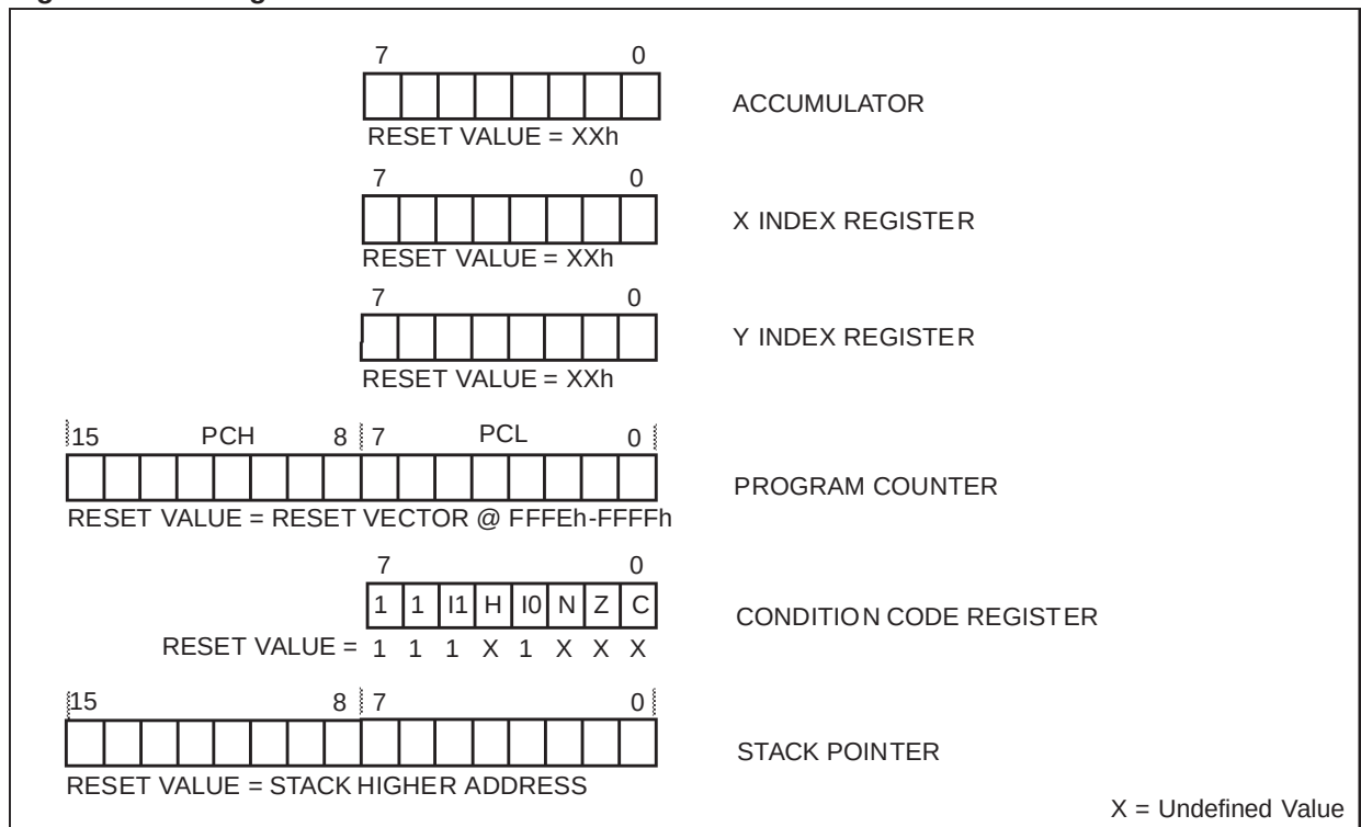
Figure 7. CPU Registers
