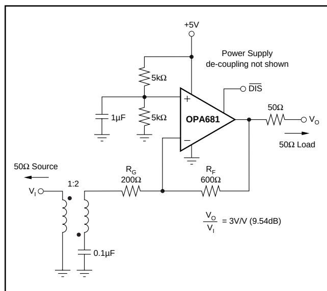
FIGURE 5. Low Noise, Single Supply, IF Amplifier.
