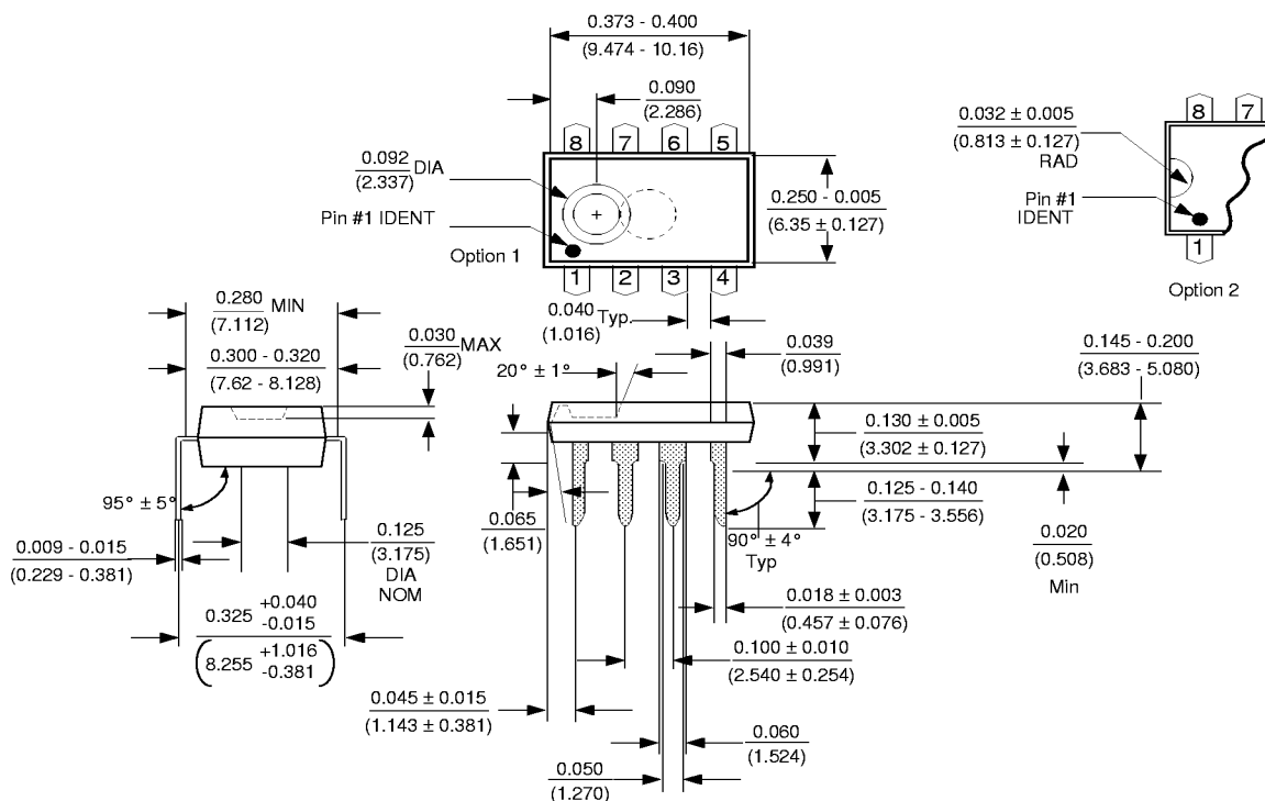
Molded Dual-In-Line Package (N) Package Number N08E
