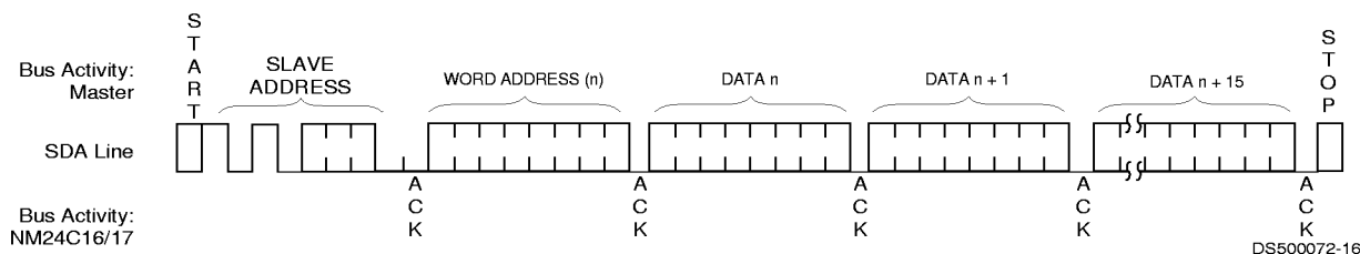
Page Write (Figure 7)
