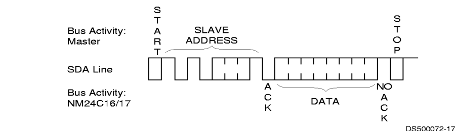
Random Read (Figure 9)
