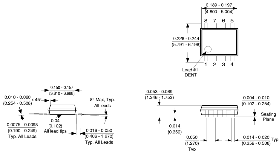
8-Pin Molded Small Outline Package (M8) Package Number M08A
