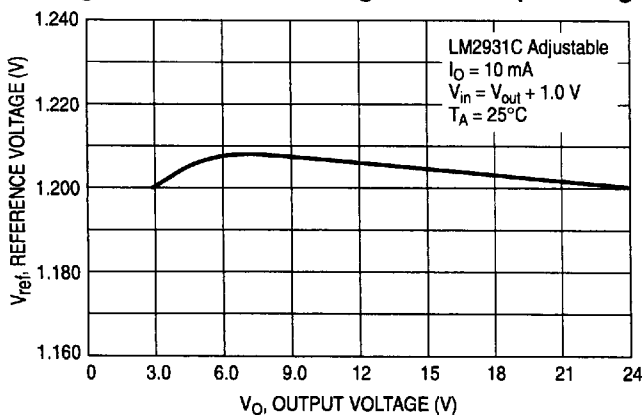
Figure 15. Reference Voltage versus Output Voltage
