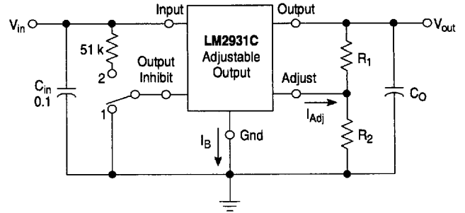
Figure 18. Adjustable Output Regulator
