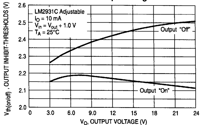
Figure 16. Output Inhibit-Thresholds versus Output Voltage
