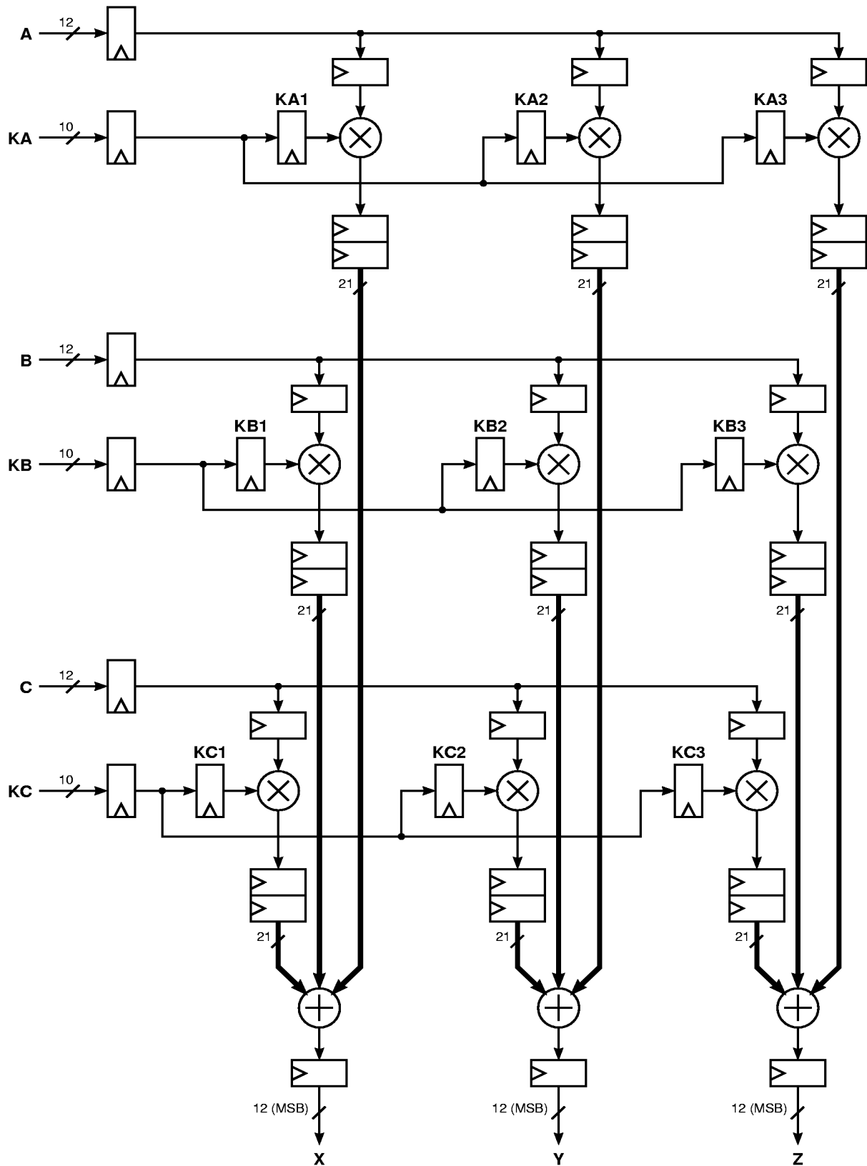
FIGURE 2. 3 x 3 MATRIX MULTIPLIER — MODE 00
