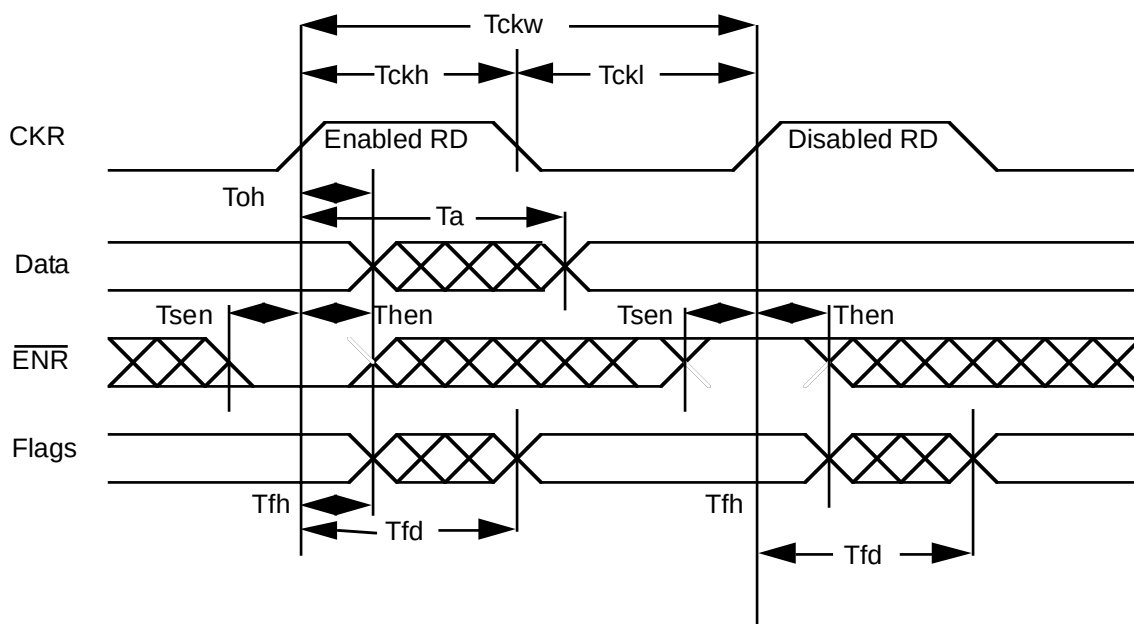
Figure 2. Read Timing
