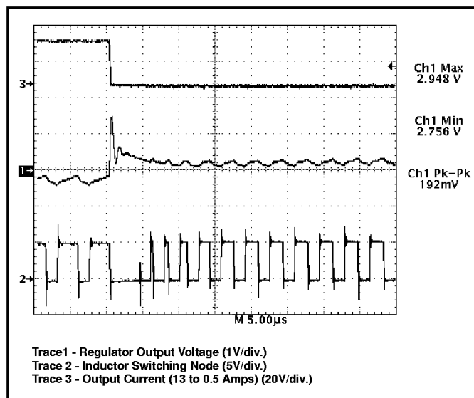
Figure 9: CS-5155 demonstration board response to 13A load turn off (output set for 2.8V). V^{2TM} control topology immediately connects inductor to ground, providing 0% duty cycle. Regulation is achieved in less than 10μs.
