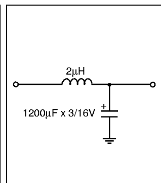
Figure 19: Input Filter
