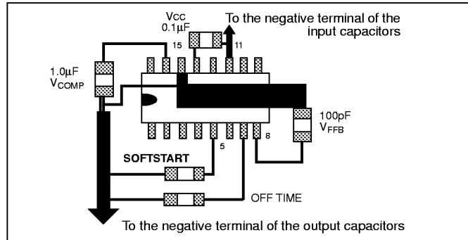
Figure 20: Layout Guidelines
