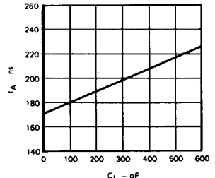
Typical t_A Versus C_L
