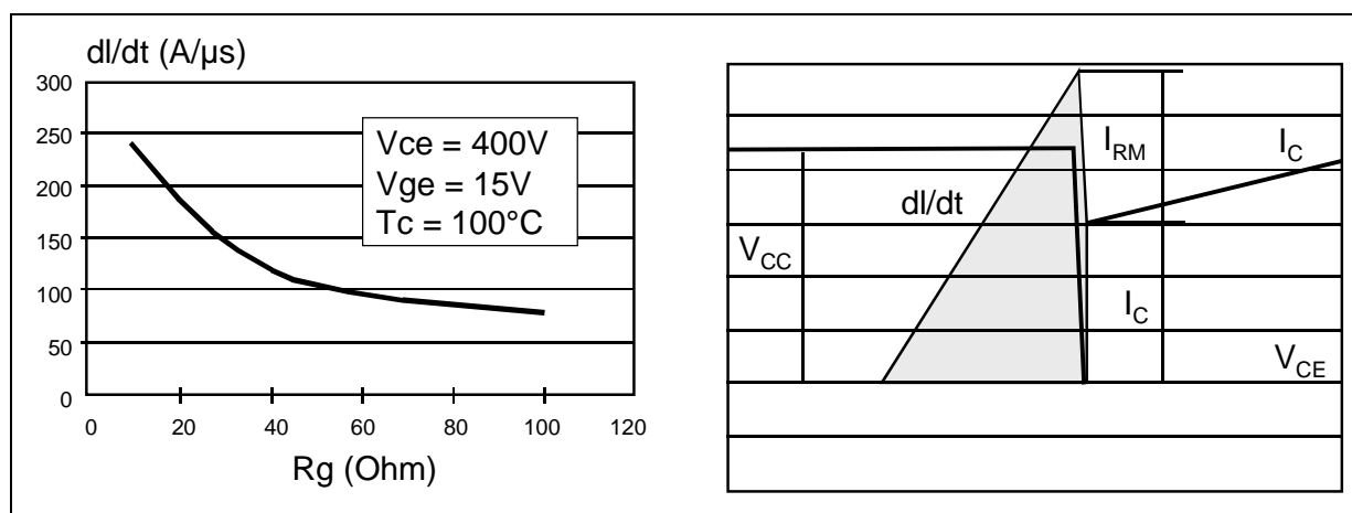
Figure 7: Rg Effect On di/dt And Energy In Turn-On
