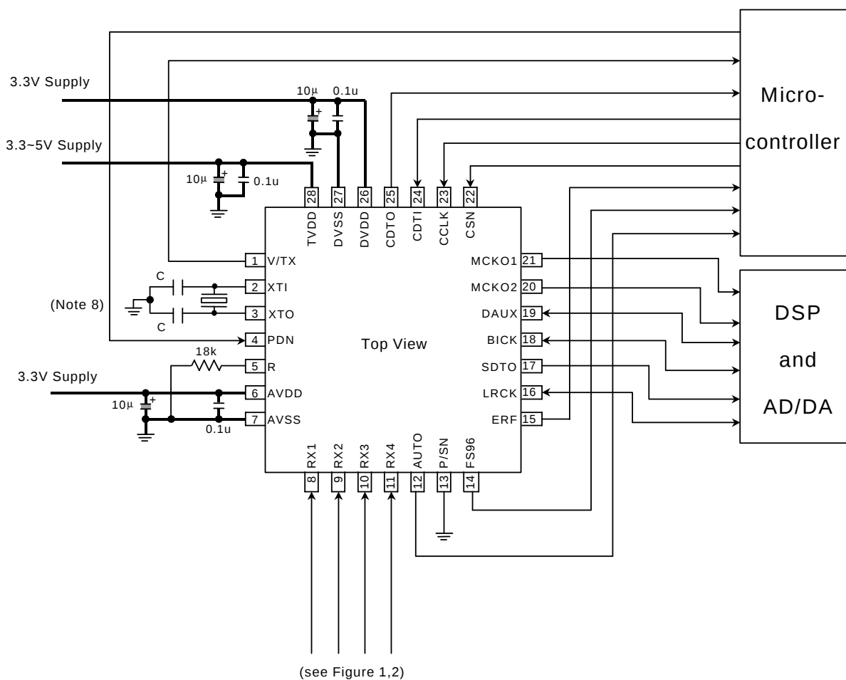
Figure 12. Typical Connection Diagram (Serial Mode)
