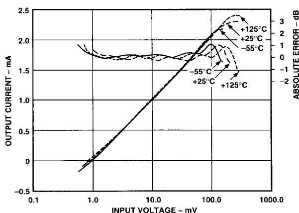
Figure 18. Logarithmic Output and Absolute Error vs. DC or Square Wave Input at T_A = -55^\circ\text{C} , +25^\circ\text{C} , and +125^\circ\text{C} , Input Direct to Pins 1 and 20
