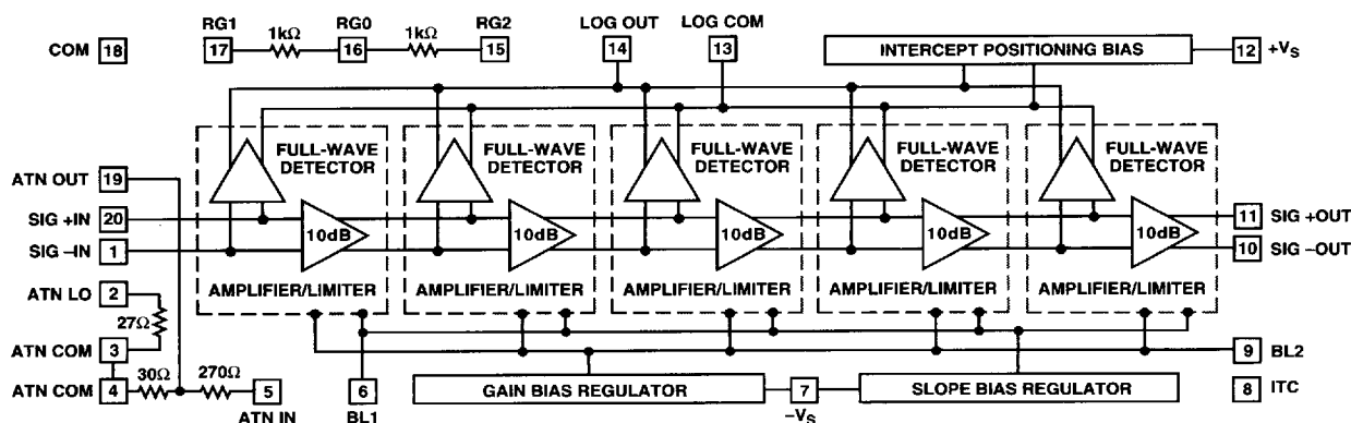
Figure 17. Block Diagram of the Complete AD641
