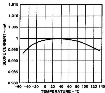
Figure 1. Slope Current, I_V , vs. Temperature
