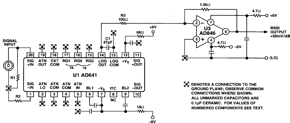
Figure 30. RSSI Using Single AD641
