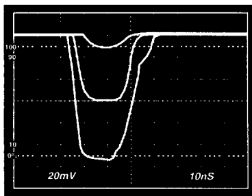
Figure 14. Baseband Pulse Response of Single AD641, Inputs of 1 mV, 10 mV and 100 mV
