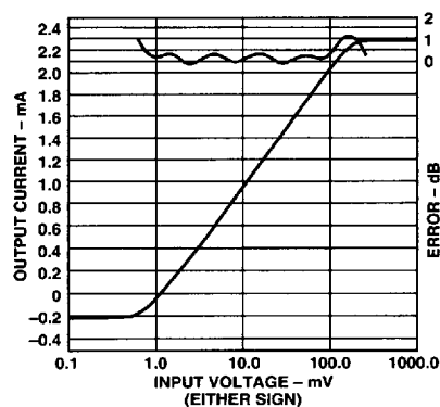
Figure 7. DC Logarithmic Transfer Function and Error Curve for Single AD641
