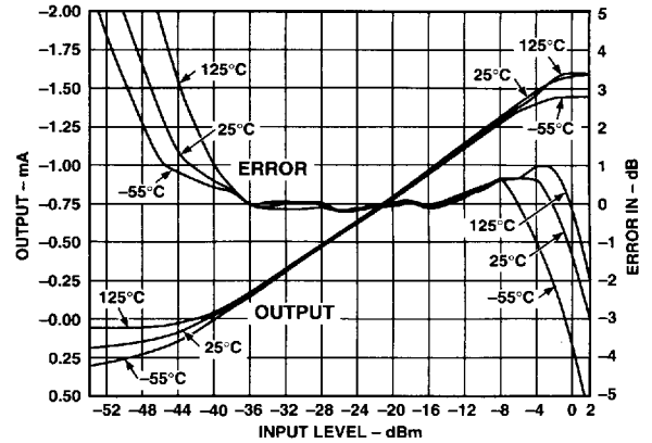
Figure 11. Logarithmic Response and Linearity at 200 MHz, T_A for T_A = -55^\circ\text{C} , +25^\circ\text{C} , +125^\circ\text{C}
