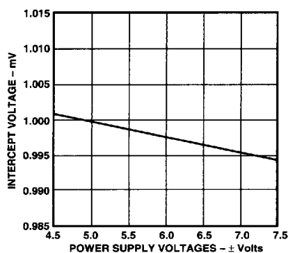
Figure 4. Intercept Voltage, V_X , vs. Supply Voltages
