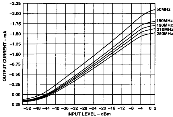
Figure 10. AC Response at 50 MHz, 150 MHz, 190 MHz, 210 MHz at 250 MHz, vs. dBm Input (Sinusoidal Input)
