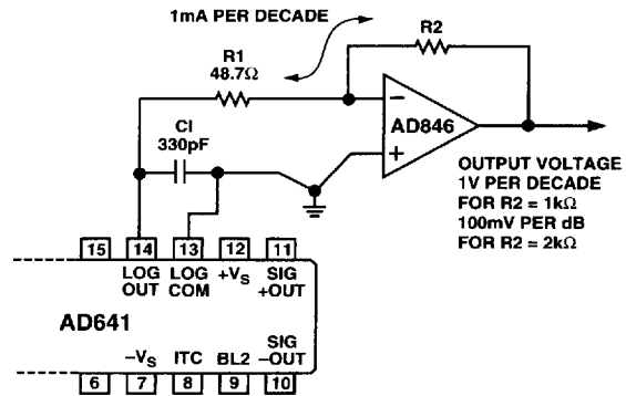
Figure 21. Using an External Op Amp to Convert the AD641 Output Current to a Buffered Voltage Output
