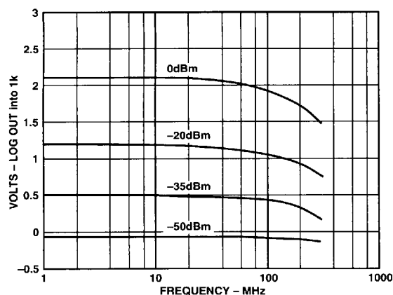
Figure 31. Single AD641 RSSI vs. Frequency
