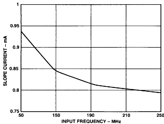
Figure 12. Slope Current, I_V , vs. Input Frequency
