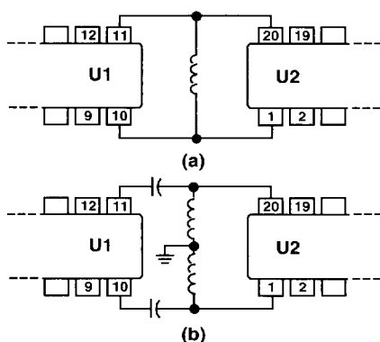
Figure 28. Two Methods for AC Coupling AD641s
