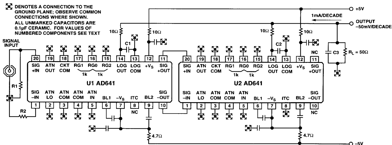
Figure 27. Basic Connections for Cascaded AD641s
