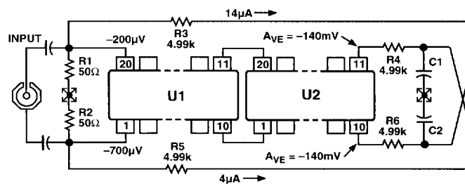
Figure 29. Feedback Offset Correction Network
