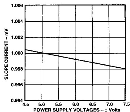
Figure 3. Slope Current, I_V , vs. Supply Voltages
