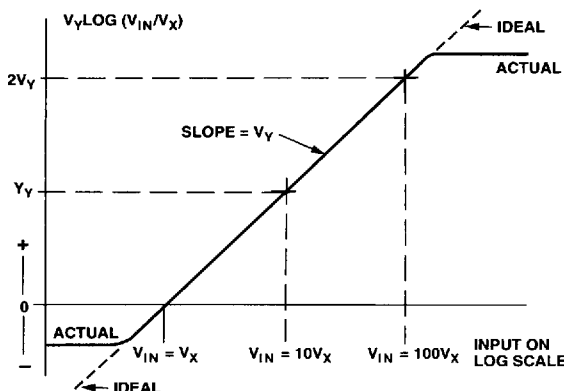
Figure 20. Basic DC Transfer Function of the AD641
