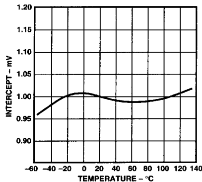
Figure 2. Intercept Voltage, V_X , vs. Temperature
