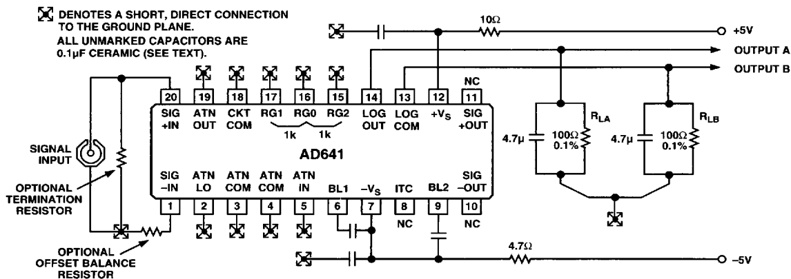
Figure 24. Connections for a Single AD641 to Verify Basic Performance
