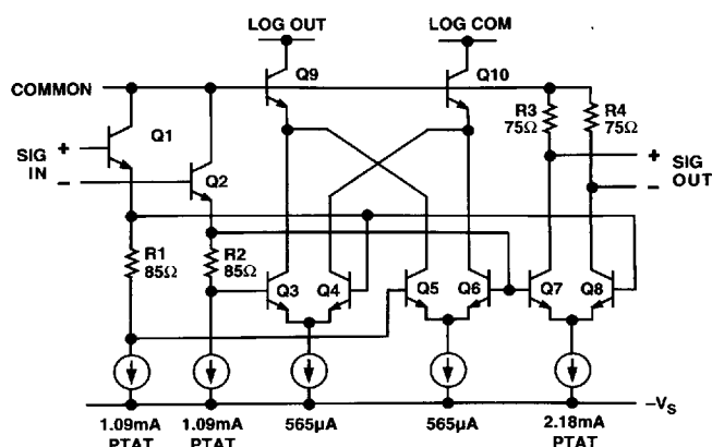
Figure 16. Simplified Schematic of a Single AD641 Stage
