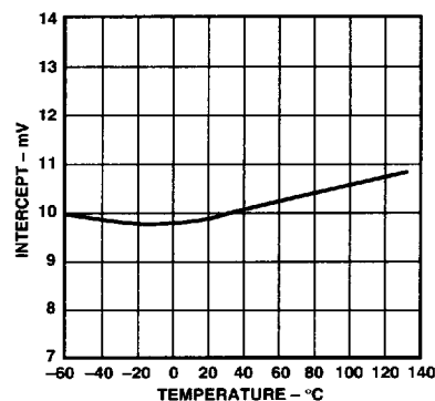
Figure 5. Intercept Voltage (Using Attenuator) vs. Temperature
