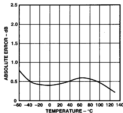
Figure 8. Absolute Error vs. Temperature, V_{IN} = \pm 1 \text{ mV to } \pm 100 \text{ mV}
