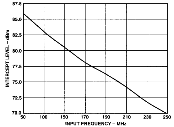
Figure 13. Intercept Level (dBm) vs. Frequency (Cascaded AD641s—Sinusoidal Input)
