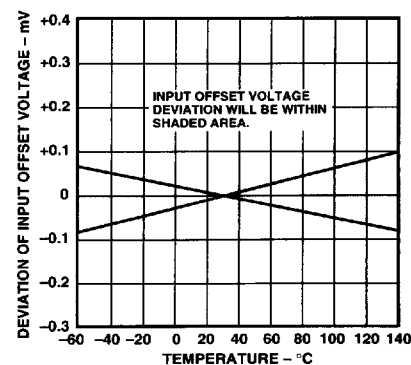
Figure 6. Input Offset Voltage Deviation vs. Temperature
