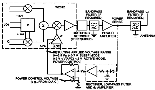
Figure 24. Simplified Transmit Power Control Concept
