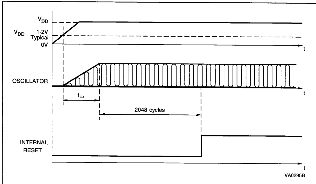
Figure 30. Power-on-Reset
