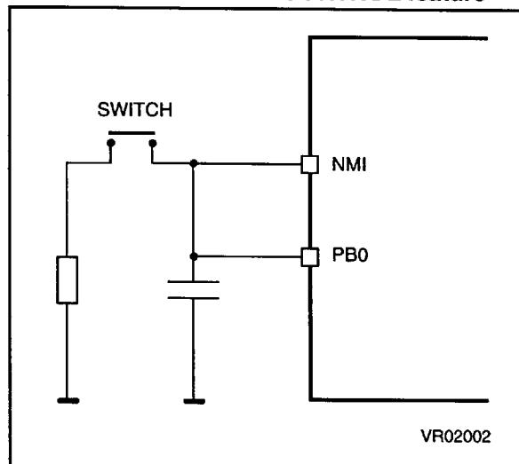
Figure 20. A typical circuit making use of the EXTERNAL STOP MODE CONTROL feature
