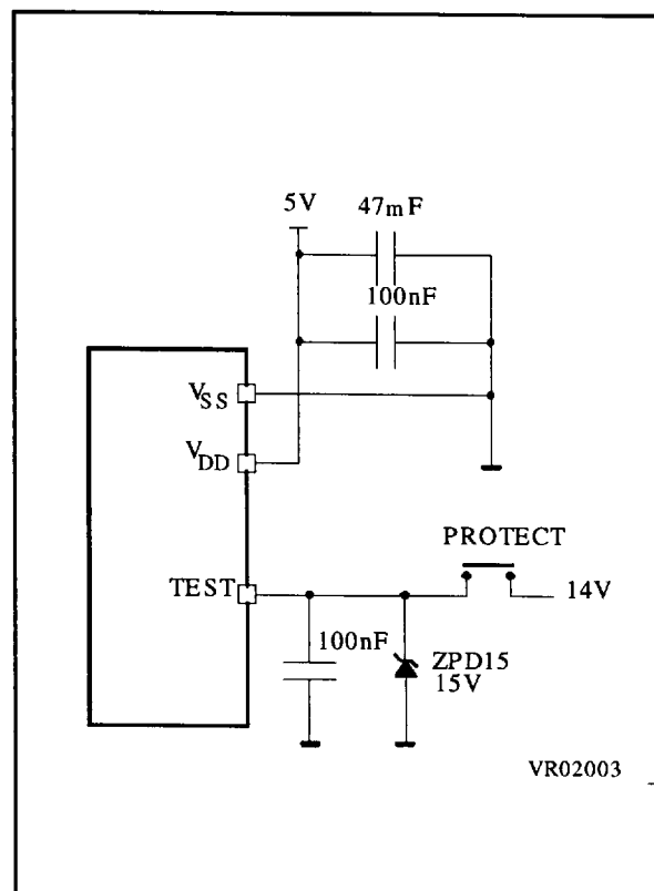
Figure 34. Programming Circuit
