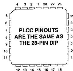
28-Pin PLCC
