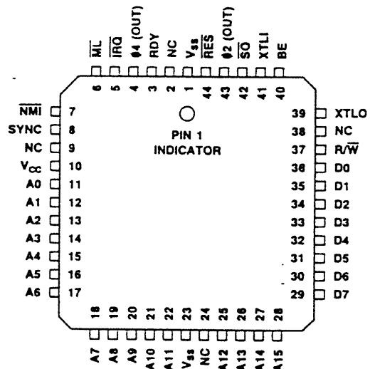
44-PIN PLCC
