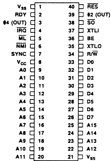
40-PIN DIP
