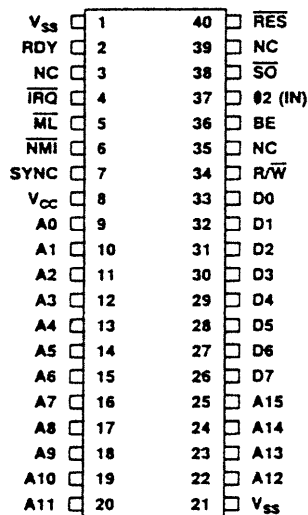
40-PIN DIP
