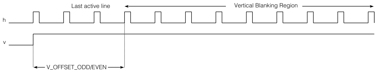
Fig. 3 V_Offset Definition
