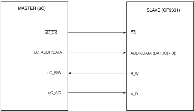
Fig. 10 Host Interface Parallel Mode
