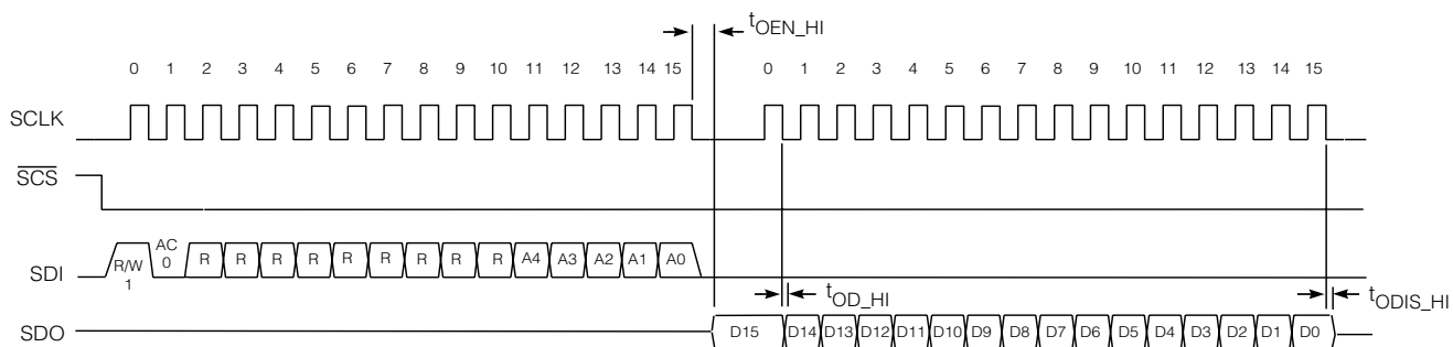
Fig. 9 Read Cycle
