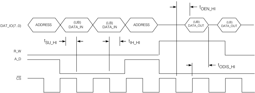
Fig. 12 Write Cycle to the Parallel Interface
