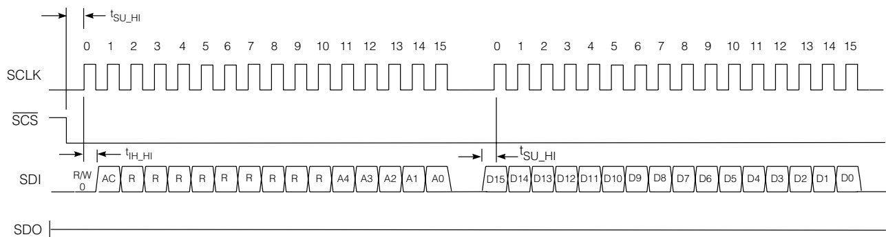
Fig. 8 Write Cycle
