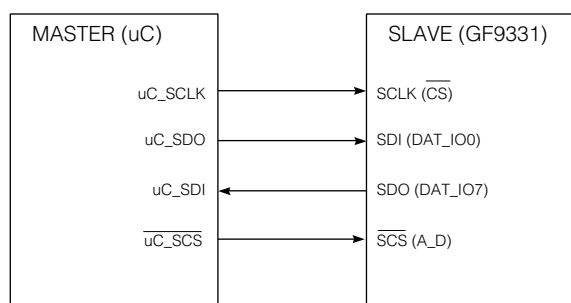
Fig.5 Host Interface Serial Mode
