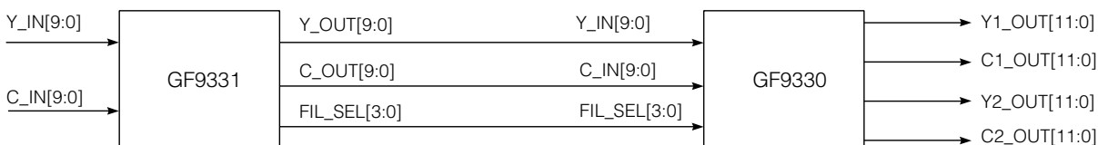
Fig. 4 Using the GF9331 with the GF9330 for Motion Adaptive De-interlacing with edge and vertical motion detection
